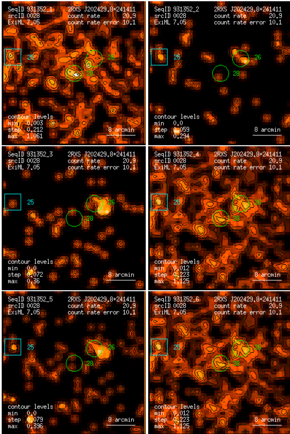
Figure 28: RASS 931352: detection 0028: band rate images, Gaussian filter: (1) PSPC channels 11 – 41, (2) 52 – 90, (3) 91 – 201, (4) 11 – 235, (5) 52 – 201, (6) 11 – 201. Broad band rates in counts/ks. Band rate contour levels in counts/ks/arcmin 2 .
