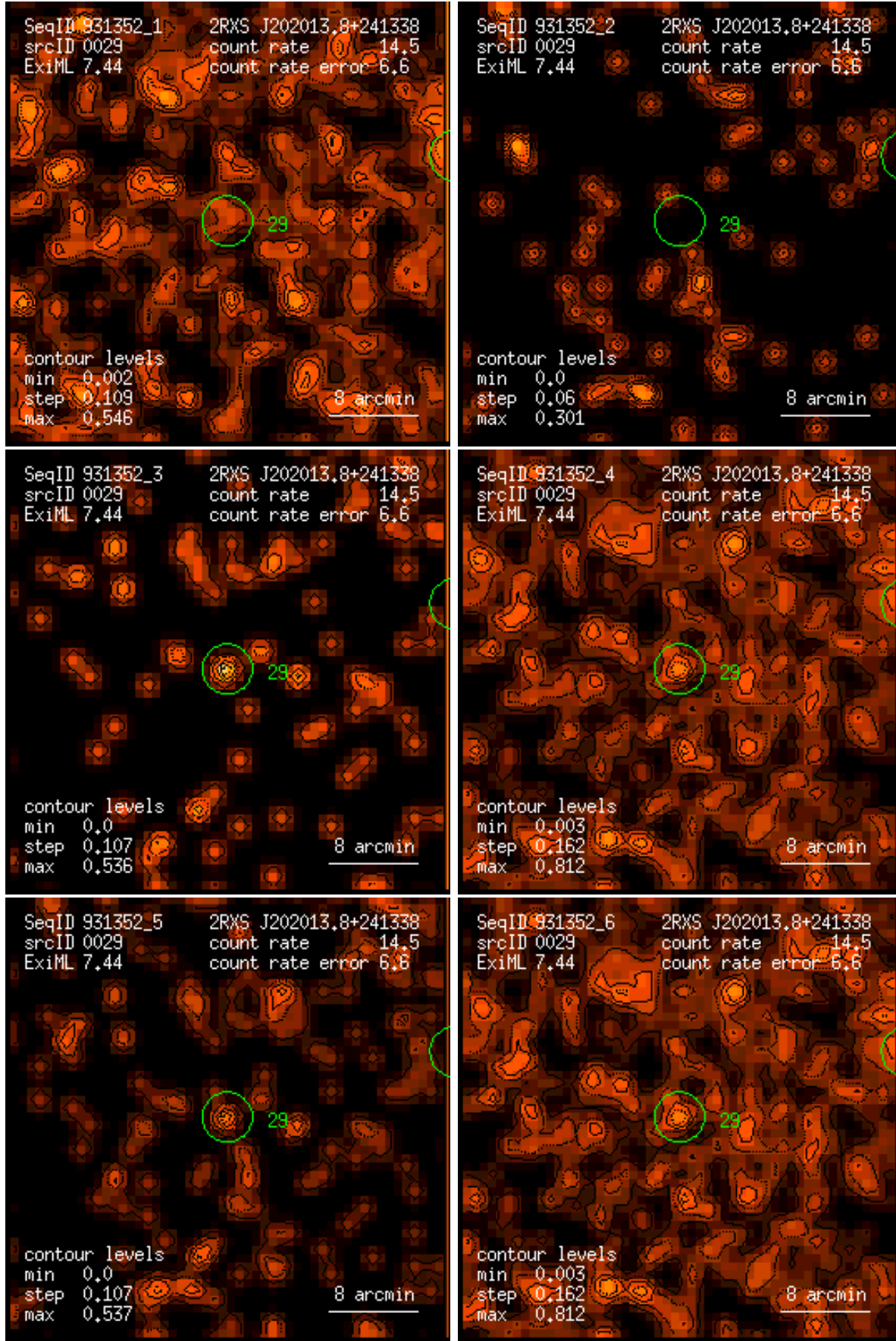
Figure 29: RASS 931352: detection 0029: band rate images, Gaussian filter: (1) PSPC channels 11 – 41, (2) 52 – 90, (3) 91 – 201, (4) 11 – 235, (5) 52 – 201, (6) 11 – 201. Broad band rates in counts/ks. Band rate contour levels in counts/ks/arcmin 2 .
