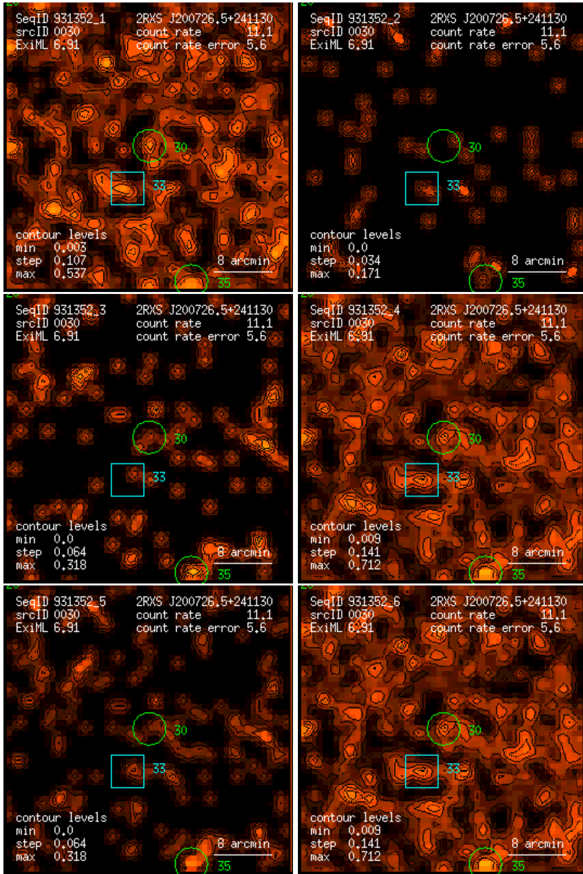
Figure 30: RASS 931352: detection 0030: band rate images, Gaussian filter: (1) PSPC channels 11 – 41, (2) 52 – 90, (3) 91 – 201, (4) 11 – 235, (5) 52 – 201, (6) 11 – 201. Broad band rates in counts/ks. Band rate contour levels in counts/ks/arcmin 2 .
