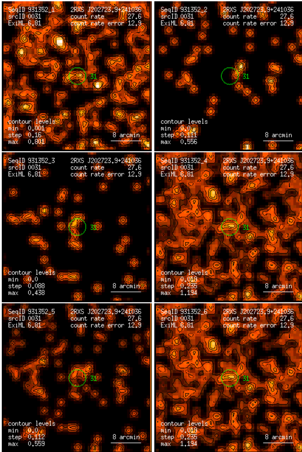
Figure 31: RASS 931352: detection 0031: band rate images, Gaussian filter: (1) PSPC channels 11 – 41, (2) 52 – 90, (3) 91 – 201, (4) 11 – 235, (5) 52 – 201, (6) 11 – 201. Broad band rates in counts/ks. Band rate contour levels in counts/ks/arcmin 2 .
