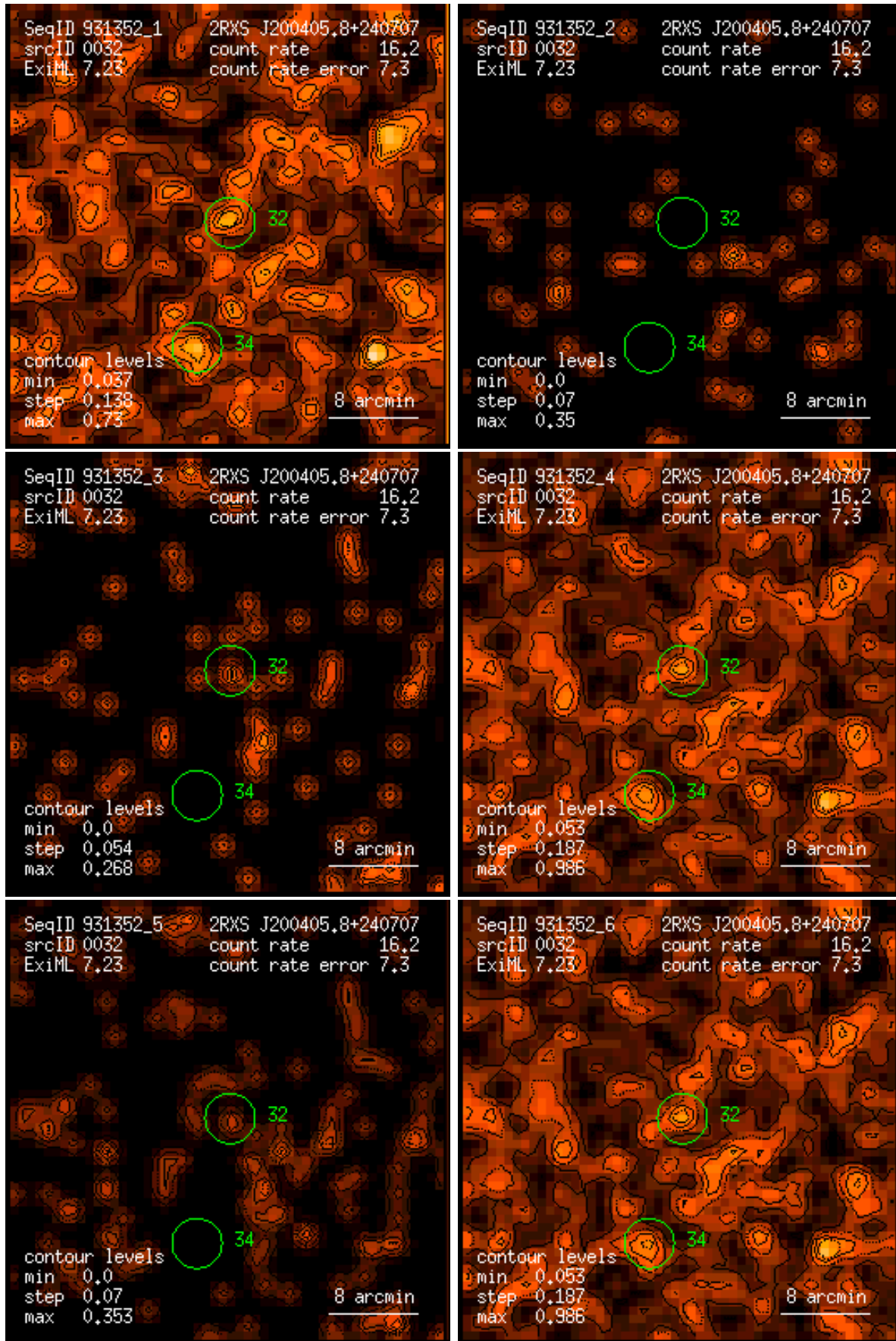
Figure 32: RASS 931352: detection 0032: band rate images, Gaussian filter: (1) PSPC channels 11 – 41, (2) 52 – 90, (3) 91 – 201, (4) 11 – 235, (5) 52 – 201, (6) 11 – 201. Broad band rates in counts/ks. Band rate contour levels in counts/ks/arcmin 2 .
