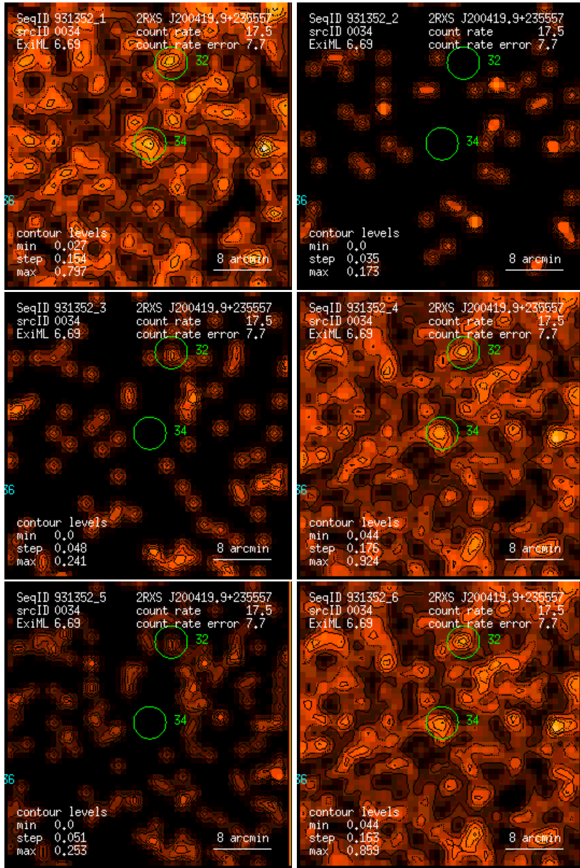
Figure 34: RASS 931352: detection 0034: band rate images, Gaussian filter: (1) PSPC channels 11 – 41, (2) 52 – 90, (3) 91 – 201, (4) 11 – 235, (5) 52 – 201, (6) 11 – 201. Broad band rates in counts/ks. Band rate contour levels in counts/ks/arcmin 2 .
