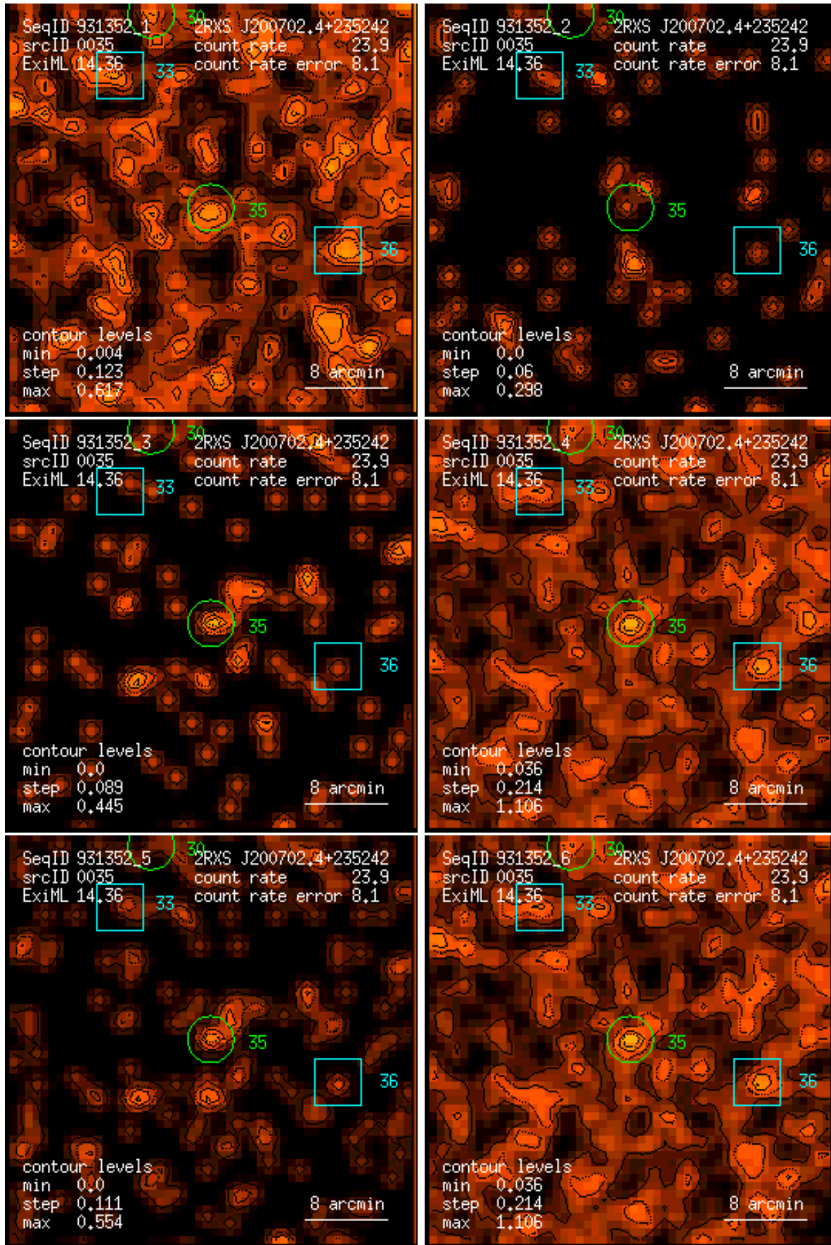
Figure 35: RASS 931352: detection 0035: band rate images, Gaussian filter: (1) PSPC channels 11 – 41, (2) 52 – 90, (3) 91 – 201, (4) 11 – 235, (5) 52 – 201, (6) 11 – 201. Broad band rates in counts/ks. Band rate contour levels in counts/ks/arcmin 2 .
