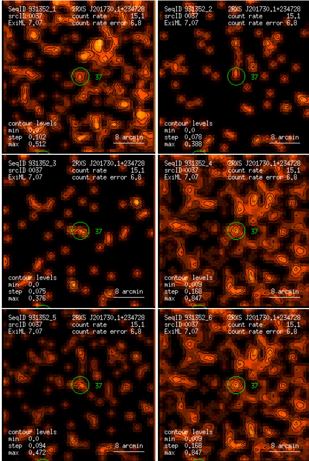
Figure 37: RASS 931352: detection 0037: band rate images, Gaussian filter: (1) PSPC channels 11 – 41, (2) 52 – 90, (3) 91 – 201, (4) 11 – 235, (5) 52 – 201, (6) 11 – 201. Broad band rates in counts/ks. Band rate contour levels in counts/ks/arcmin 2 .
