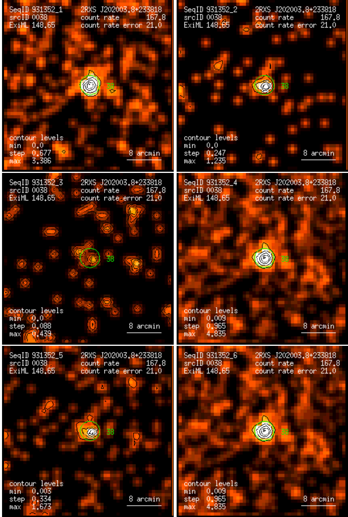
Figure 38: RASS 931352: detection 0038: band rate images, Gaussian filter: (1) PSPC channels 11 – 41, (2) 52 – 90, (3) 91 – 201, (4) 11 – 235, (5) 52 – 201, (6) 11 – 201. Broad band rates in counts/ks. Band rate contour levels in counts/ks/arcmin 2 .
