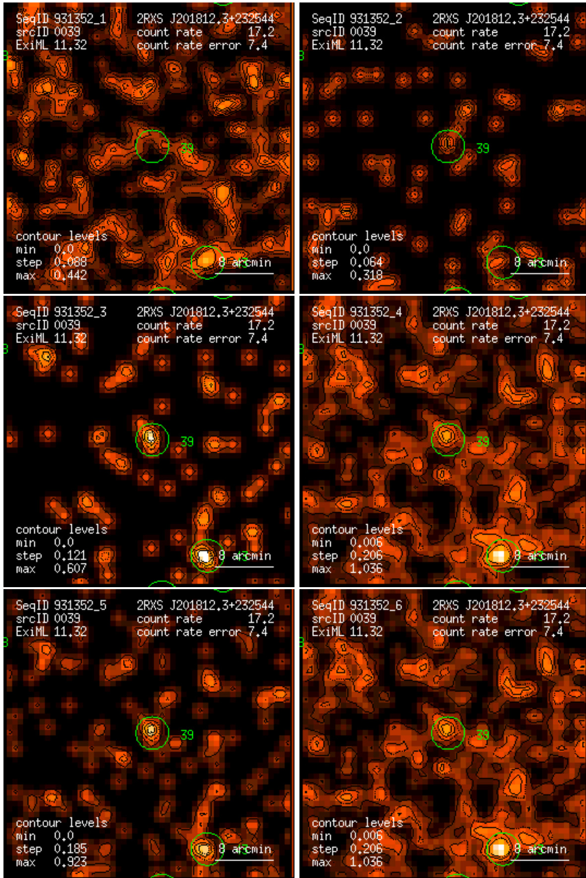
Figure 39: RASS 931352: detection 0039: band rate images, Gaussian filter: (1) PSPC channels 11 – 41, (2) 52 – 90, (3) 91 – 201, (4) 11 – 235, (5) 52 – 201, (6) 11 – 201. Broad band rates in counts/ks. Band rate contour levels in counts/ks/arcmin 2 .
