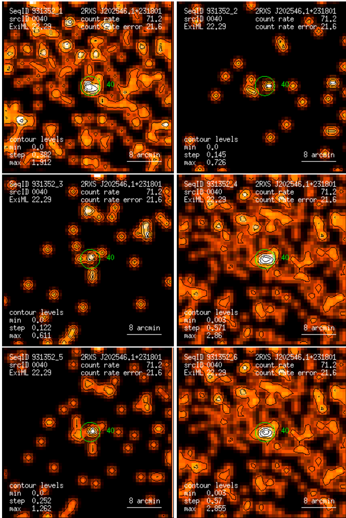
Figure 40: RASS 931352: detection 0040: band rate images, Gaussian filter: (1) PSPC channels 11 – 41, (2) 52 – 90, (3) 91 – 201, (4) 11 – 235, (5) 52 – 201, (6) 11 – 201. Broad band rates in counts/ks. Band rate contour levels in counts/ks/arcmin 2 .
