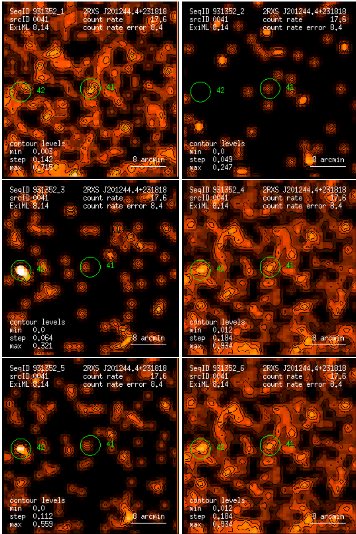
Figure 41: RASS 931352: detection 0041: band rate images, Gaussian filter: (1) PSPC channels 11 – 41, (2) 52 – 90, (3) 91 – 201, (4) 11 – 235, (5) 52 – 201, (6) 11 – 201. Broad band rates in counts/ks. Band rate contour levels in counts/ks/arcmin 2 .
