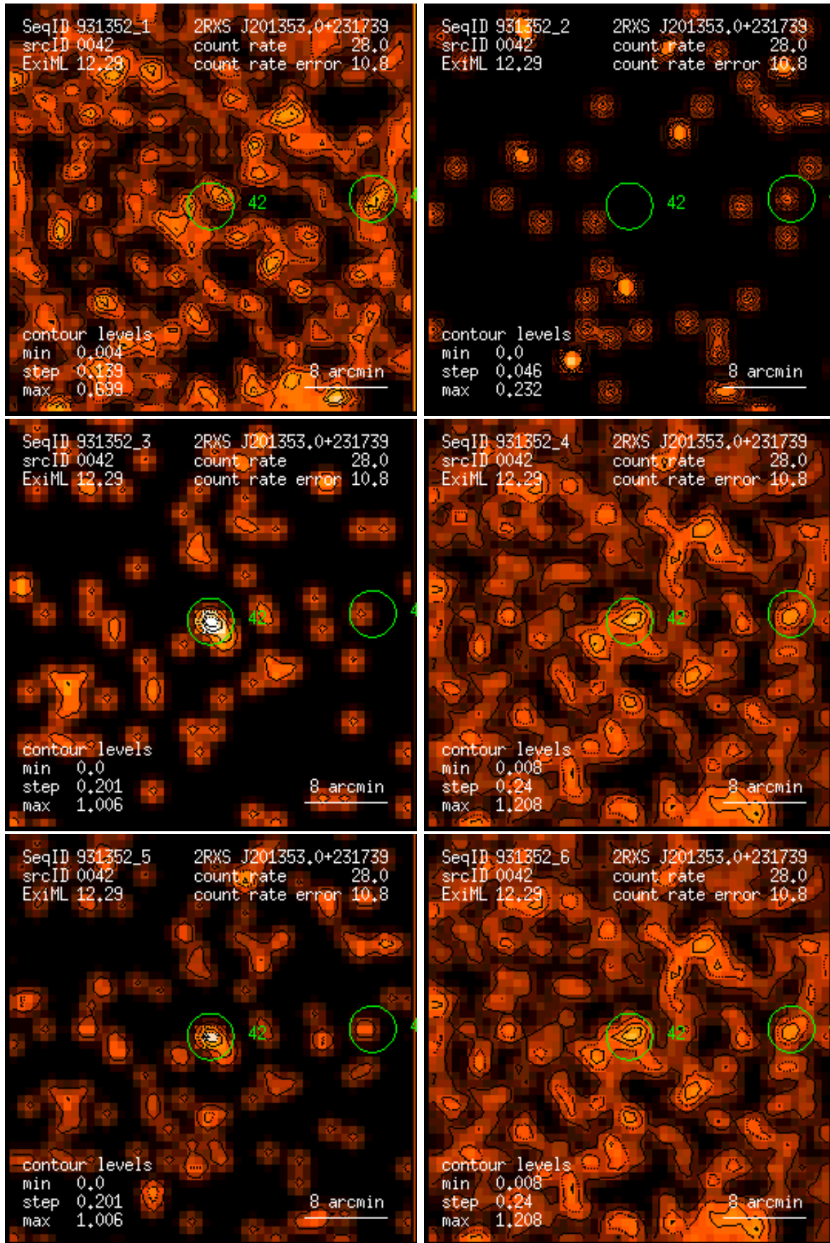
Figure 42: RASS 931352: detection 0042: band rate images, Gaussian filter: (1) PSPC channels 11 – 41, (2) 52 – 90, (3) 91 – 201, (4) 11 – 235, (5) 52 – 201, (6) 11 – 201. Broad band rates in counts/ks. Band rate contour levels in counts/ks/arcmin 2 .
