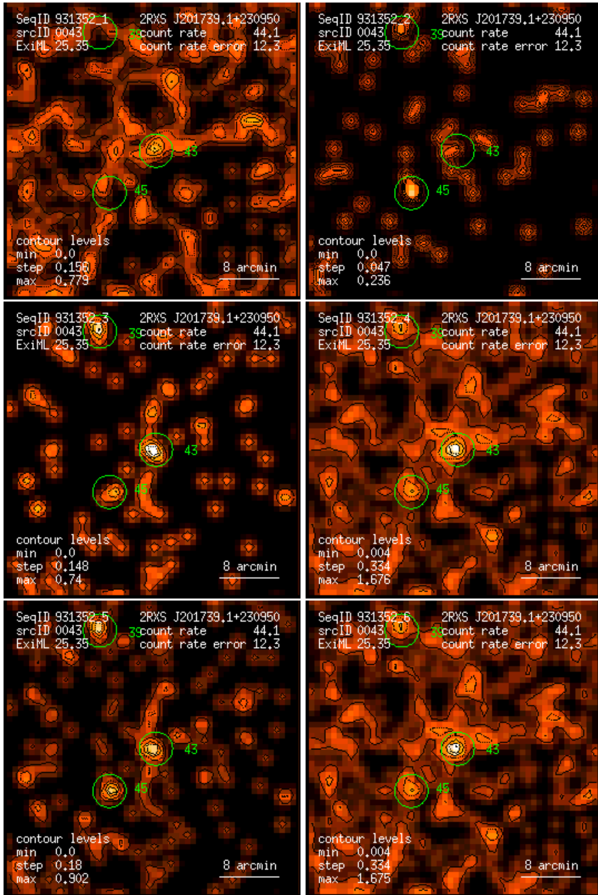
Figure 43: RASS 931352: detection 0043: band rate images, Gaussian filter: (1) PSPC channels 11 – 41, (2) 52 – 90, (3) 91 – 201, (4) 11 – 235, (5) 52 – 201, (6) 11 – 201. Broad band rates in counts/ks. Band rate contour levels in counts/ks/arcmin 2 .
