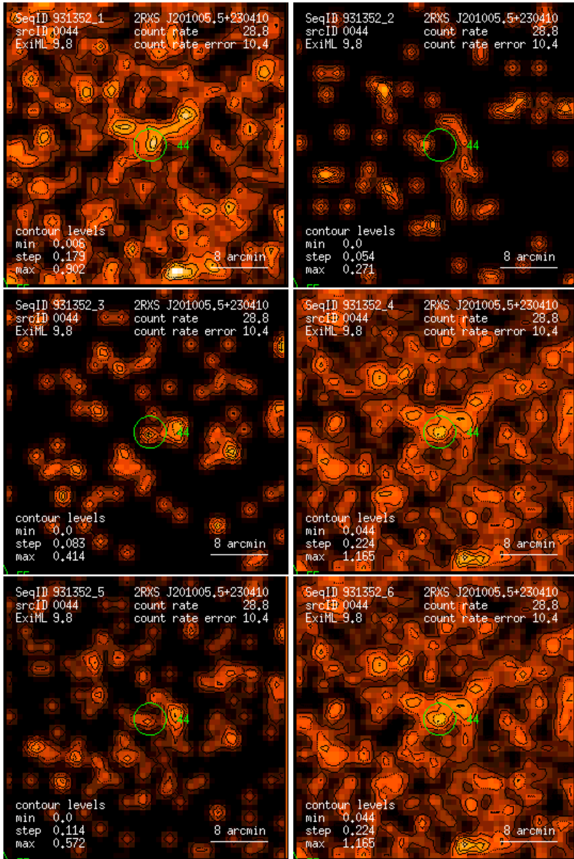
Figure 44: RASS 931352: detection 0044: band rate images, Gaussian filter: (1) PSPC channels 11 – 41, (2) 52 – 90, (3) 91 – 201, (4) 11 – 235, (5) 52 – 201, (6) 11 – 201. Broad band rates in counts/ks. Band rate contour levels in counts/ks/arcmin 2 .
