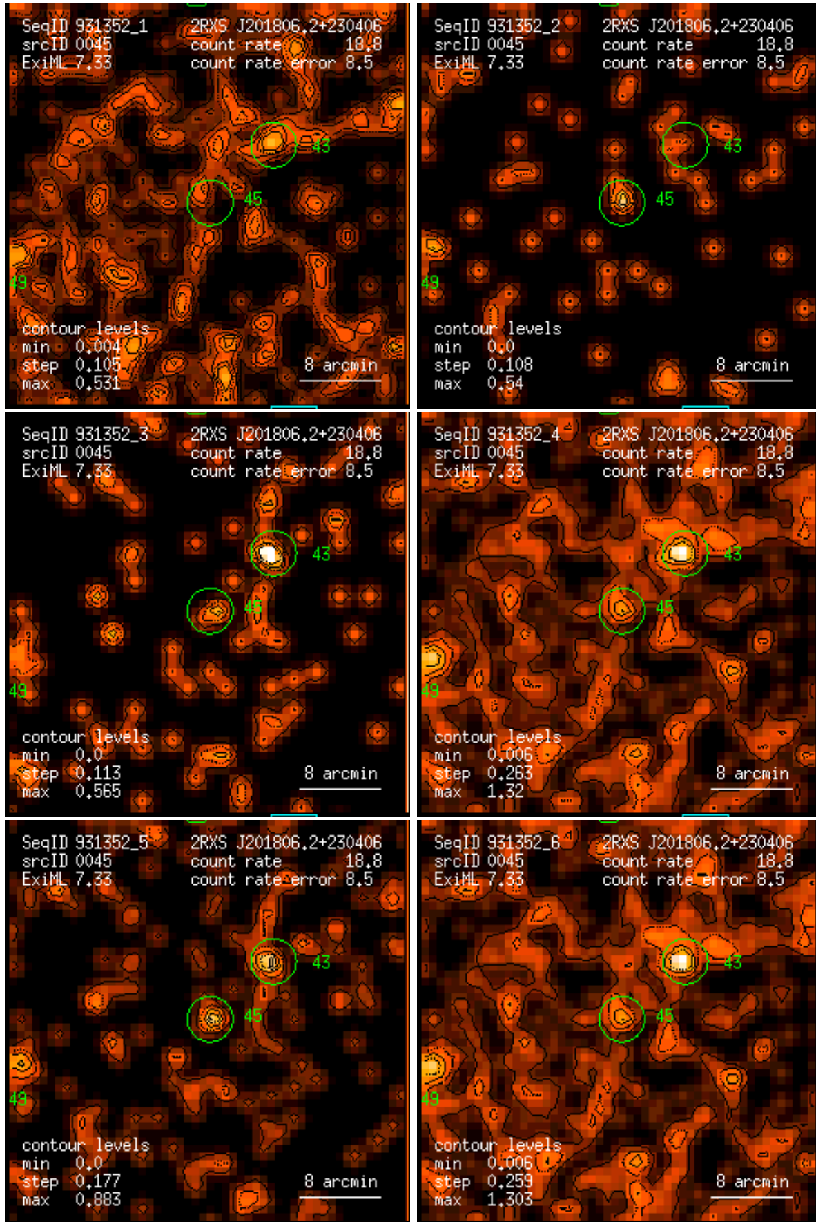
Figure 45: RASS 931352: detection 0045: band rate images, Gaussian filter: (1) PSPC channels 11 – 41, (2) 52 – 90, (3) 91 – 201, (4) 11 – 235, (5) 52 – 201, (6) 11 – 201. Broad band rates in counts/ks. Band rate contour levels in counts/ks/arcmin 2 .
