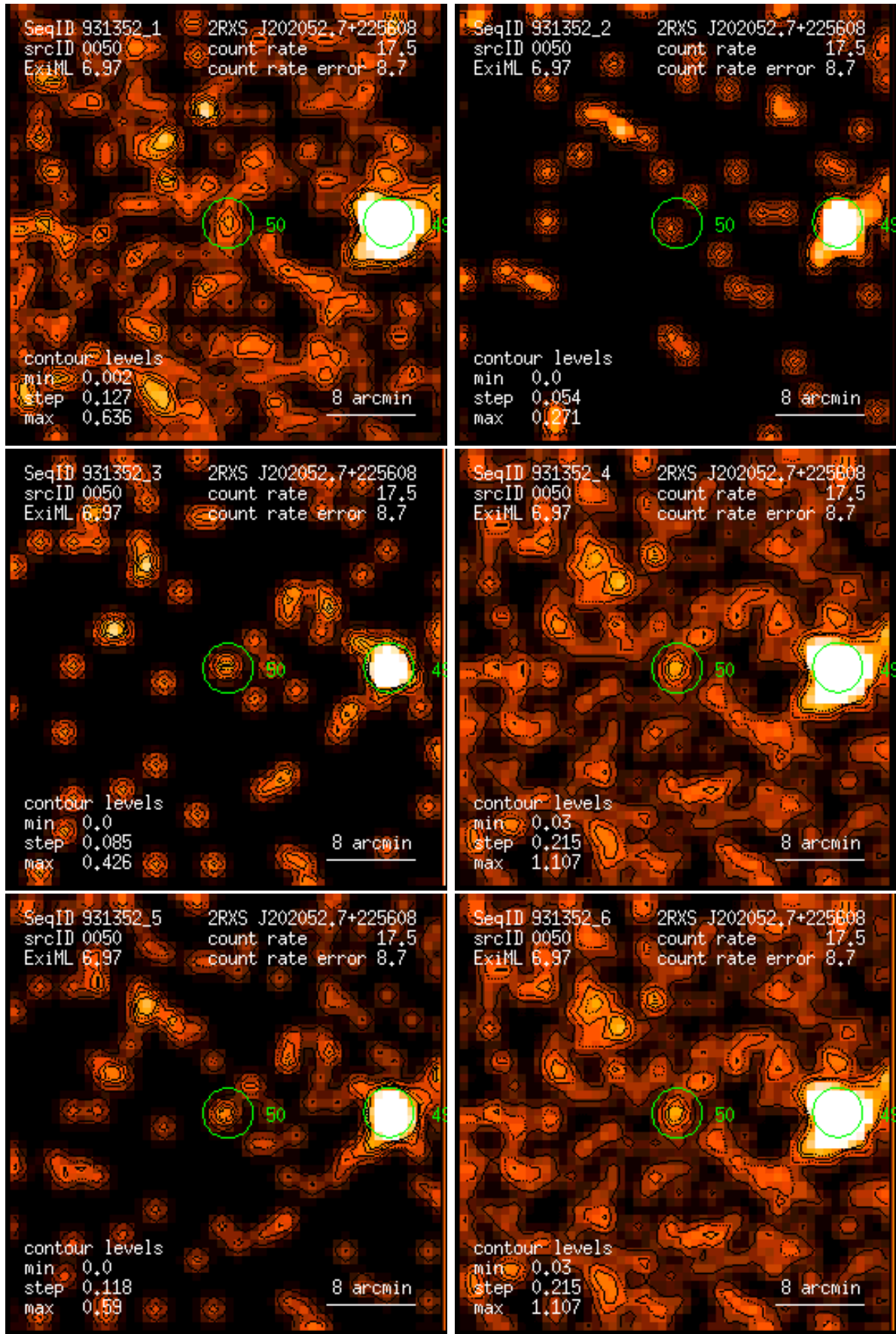
Figure 50: RASS 931352: detection 0050: band rate images, Gaussian filter: (1) PSPC channels 11 – 41, (2) 52 – 90, (3) 91 – 201, (4) 11 – 235, (5) 52 – 201, (6) 11 – 201. Broad band rates in counts/ks. Band rate contour levels in counts/ks/arcmin 2 .
