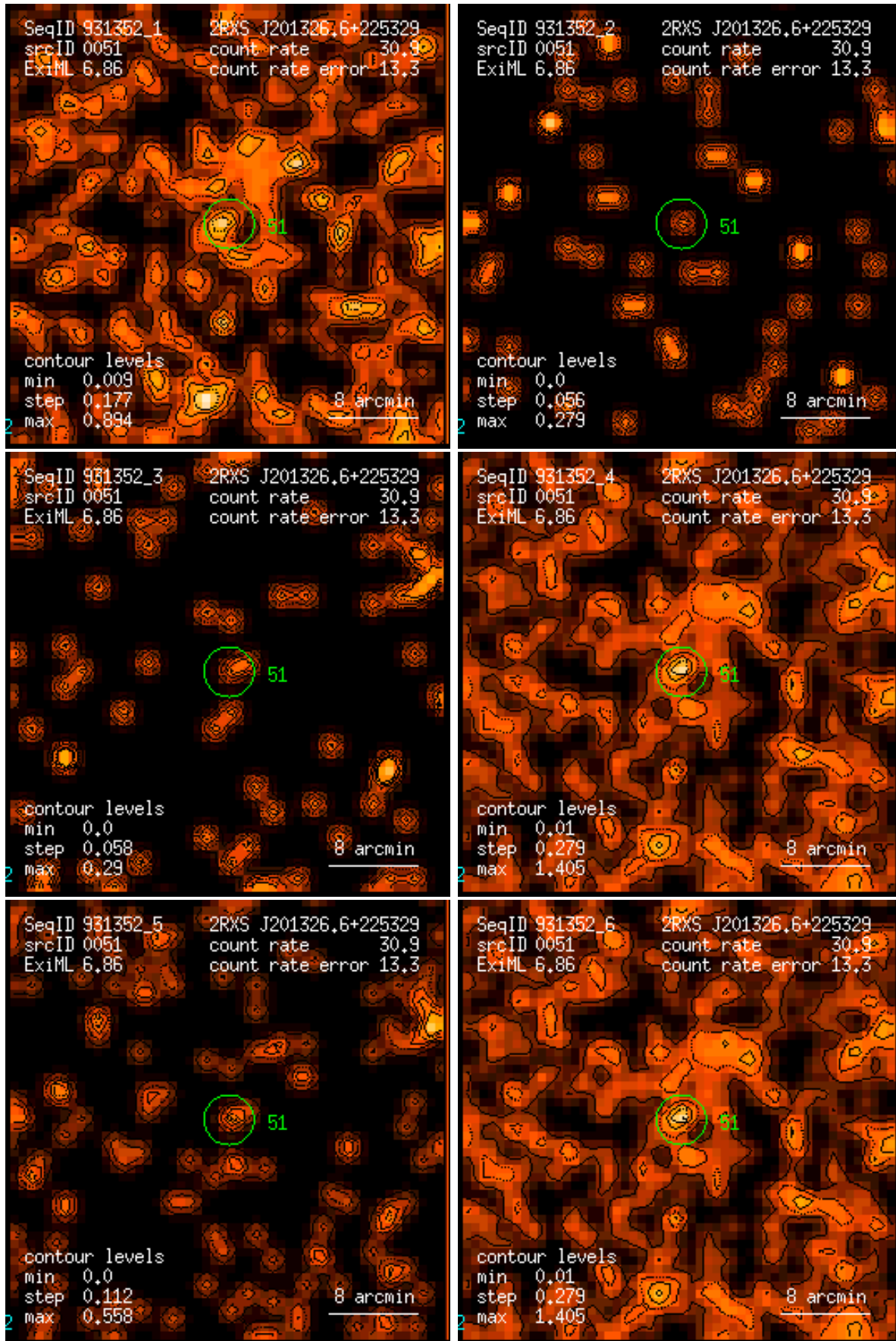
Figure 51: RASS 931352: detection 0051: band rate images, Gaussian filter: (1) PSPC channels 11 – 41, (2) 52 – 90, (3) 91 – 201, (4) 11 – 235, (5) 52 – 201, (6) 11 – 201. Broad band rates in counts/ks. Band rate contour levels in counts/ks/arcmin 2 .
