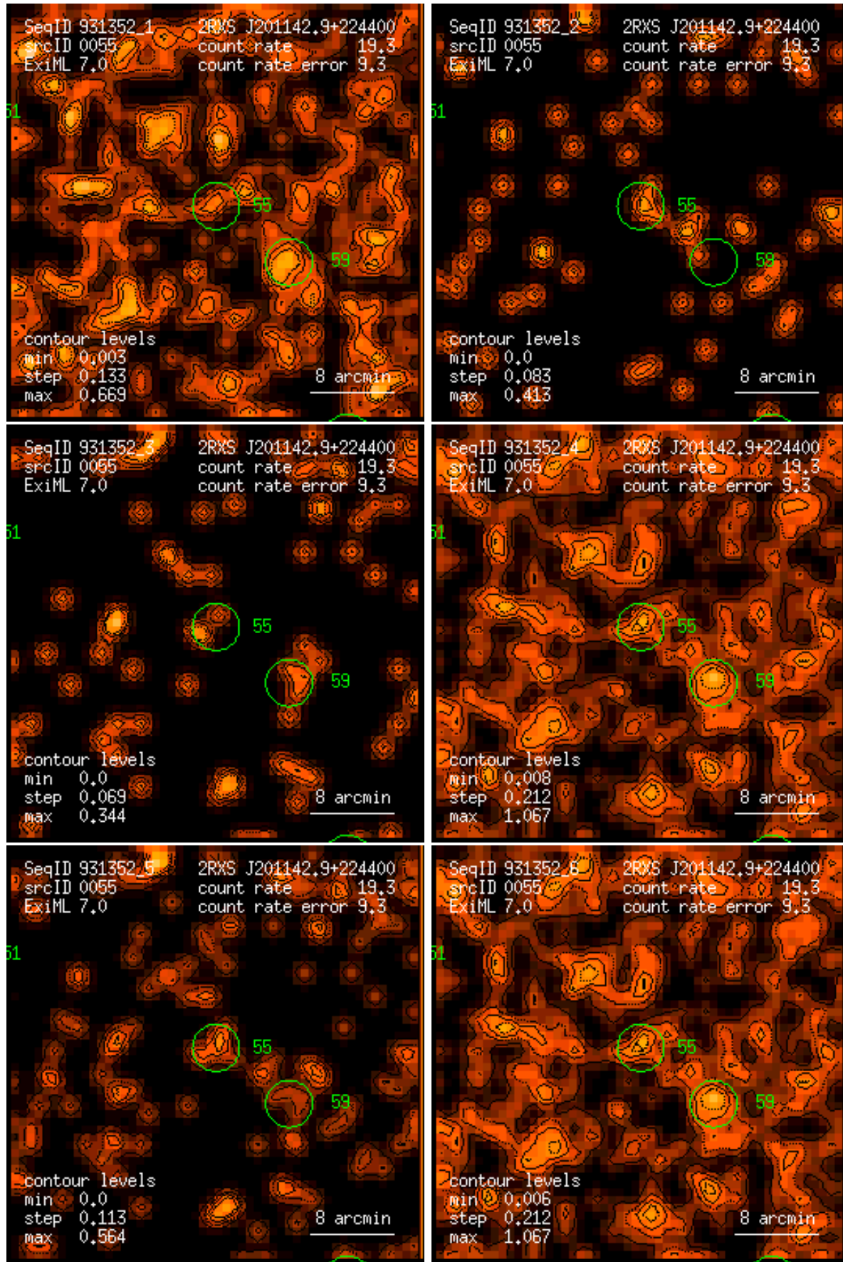
Figure 55: RASS 931352: detection 0055: band rate images, Gaussian filter: (1) PSPC channels 11 – 41, (2) 52 – 90, (3) 91 – 201, (4) 11 – 235, (5) 52 – 201, (6) 11 – 201. Broad band rates in counts/ks. Band rate contour levels in counts/ks/arcmin 2 .
