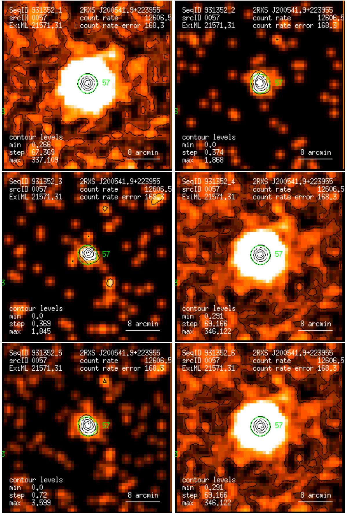
Figure 57: RASS 931352: detection 0057: band rate images, Gaussian filter: (1) PSPC channels 11 – 41, (2) 52 – 90, (3) 91 – 201, (4) 11 – 235, (5) 52 – 201, (6) 11 – 201. Broad band rates in counts/ks. Band rate contour levels in counts/ks/arcmin 2 .
