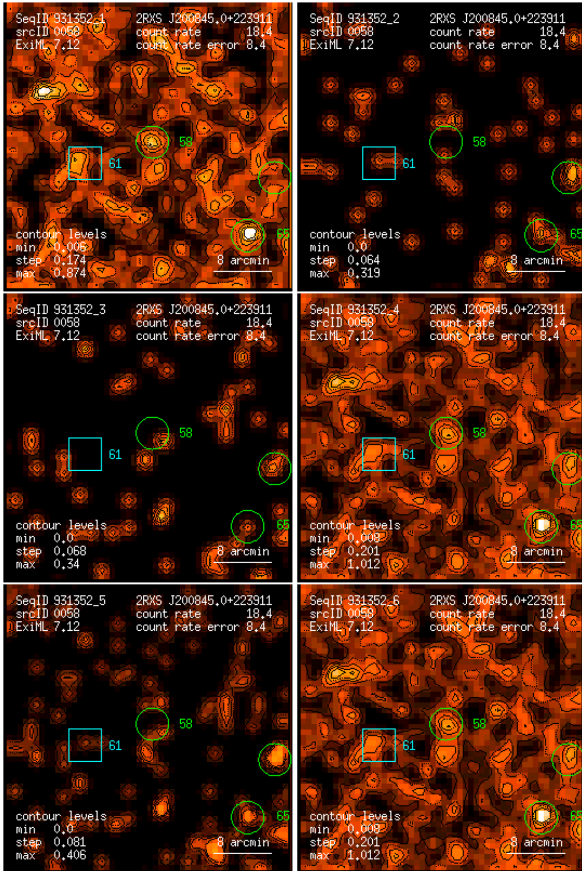
Figure 58: RASS 931352: detection 0058: band rate images, Gaussian filter: (1) PSPC channels 11 – 41, (2) 52 – 90, (3) 91 – 201, (4) 11 – 235, (5) 52 – 201, (6) 11 – 201. Broad band rates in counts/ks. Band rate contour levels in counts/ks/arcmin 2 .
