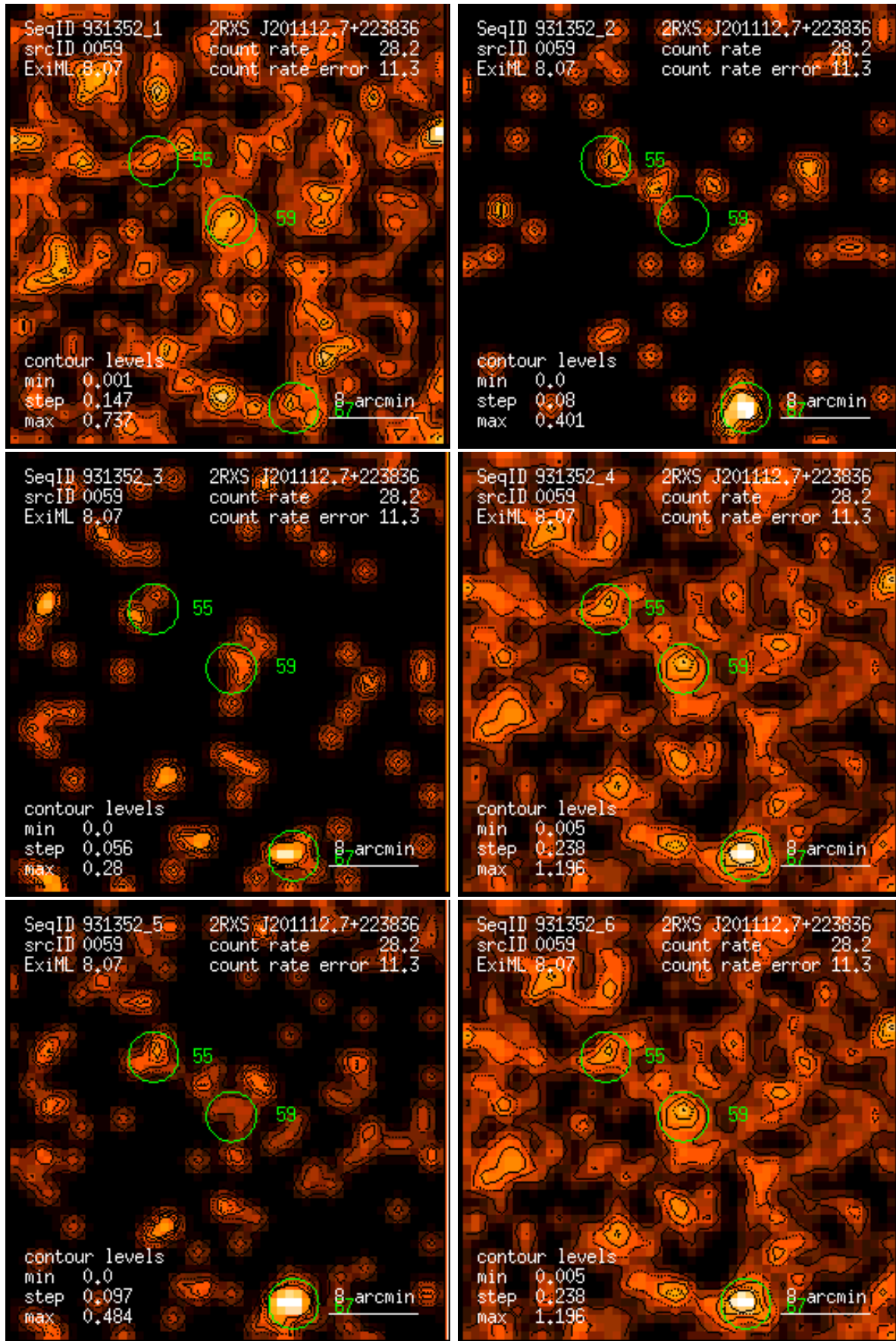
Figure 59: RASS 931352: detection 0059: band rate images, Gaussian filter: (1) PSPC channels 11 – 41, (2) 52 – 90, (3) 91 – 201, (4) 11 – 235, (5) 52 – 201, (6) 11 – 201. Broad band rates in counts/ks. Band rate contour levels in counts/ks/arcmin 2 .
