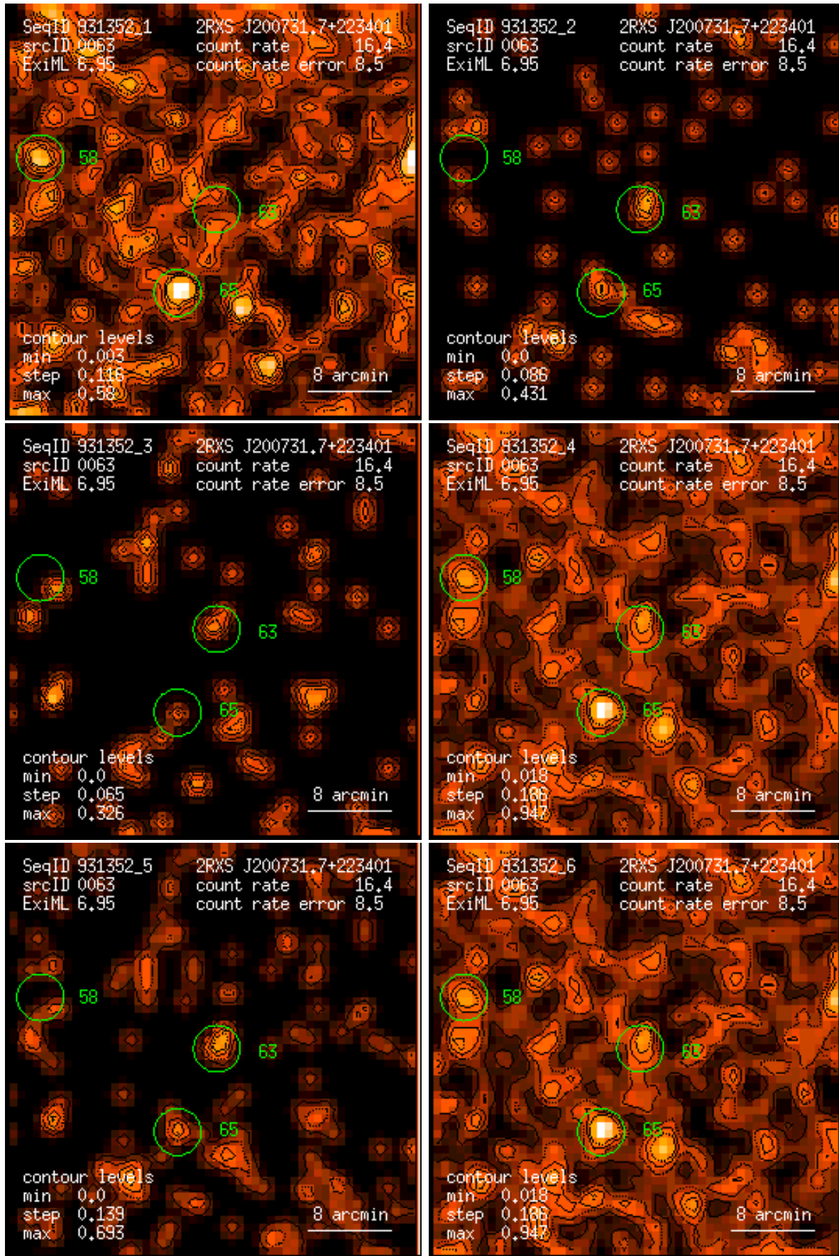
Figure 63: RASS 931352: detection 0063: band rate images, Gaussian filter: (1) PSPC channels 11 – 41, (2) 52 – 90, (3) 91 – 201, (4) 11 – 235, (5) 52 – 201, (6) 11 – 201. Broad band rates in counts/ks. Band rate contour levels in counts/ks/arcmin 2 .
