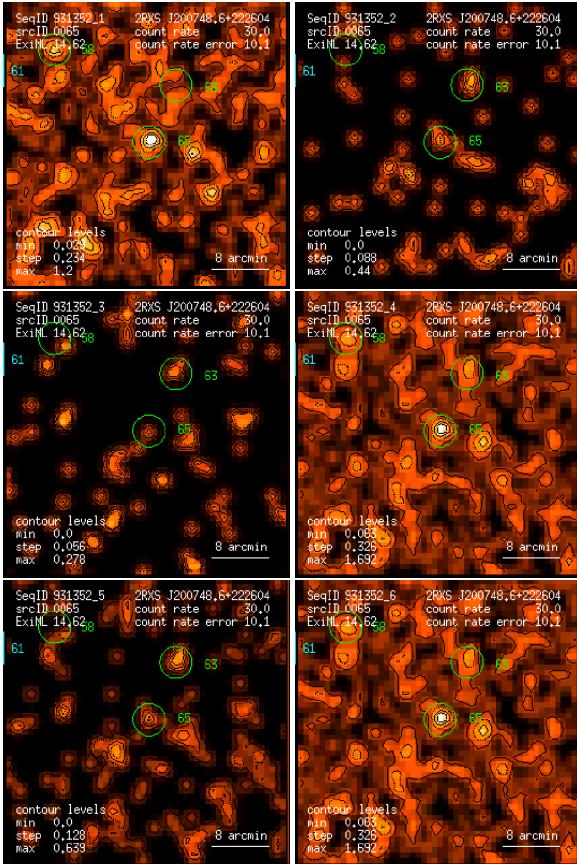
Figure 65: RASS 931352: detection 0065: band rate images, Gaussian filter: (1) PSPC channels 11 – 41, (2) 52 – 90, (3) 91 – 201, (4) 11 – 235, (5) 52 – 201, (6) 11 – 201. Broad band rates in counts/ks. Band rate contour levels in counts/ks/arcmin 2 .
