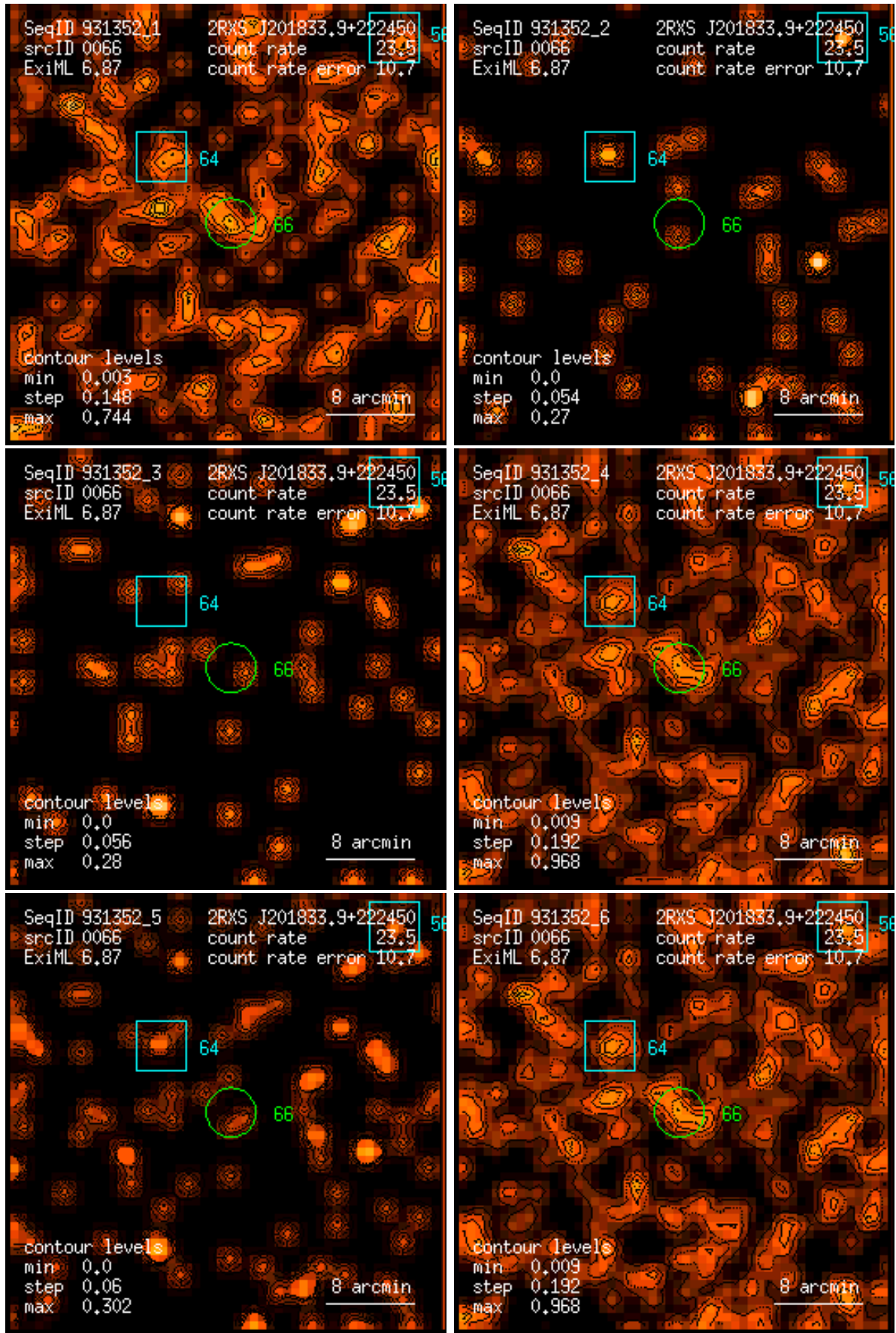
Figure 66: RASS 931352: detection 0066: band rate images, Gaussian filter: (1) PSPC channels 11 – 41, (2) 52 – 90, (3) 91 – 201, (4) 11 – 235, (5) 52 – 201, (6) 11 – 201. Broad band rates in counts/ks. Band rate contour levels in counts/ks/arcmin 2 .
