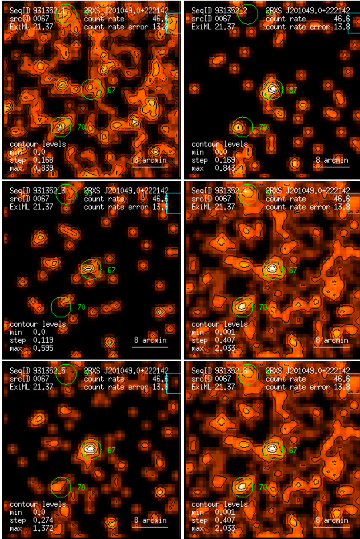
Figure 67: RASS 931352: detection 0067: band rate images, Gaussian filter: (1) PSPC channels 11 – 41, (2) 52 – 90, (3) 91 – 201, (4) 11 – 235, (5) 52 – 201, (6) 11 – 201. Broad band rates in counts/ks. Band rate contour levels in counts/ks/arcmin 2 .
