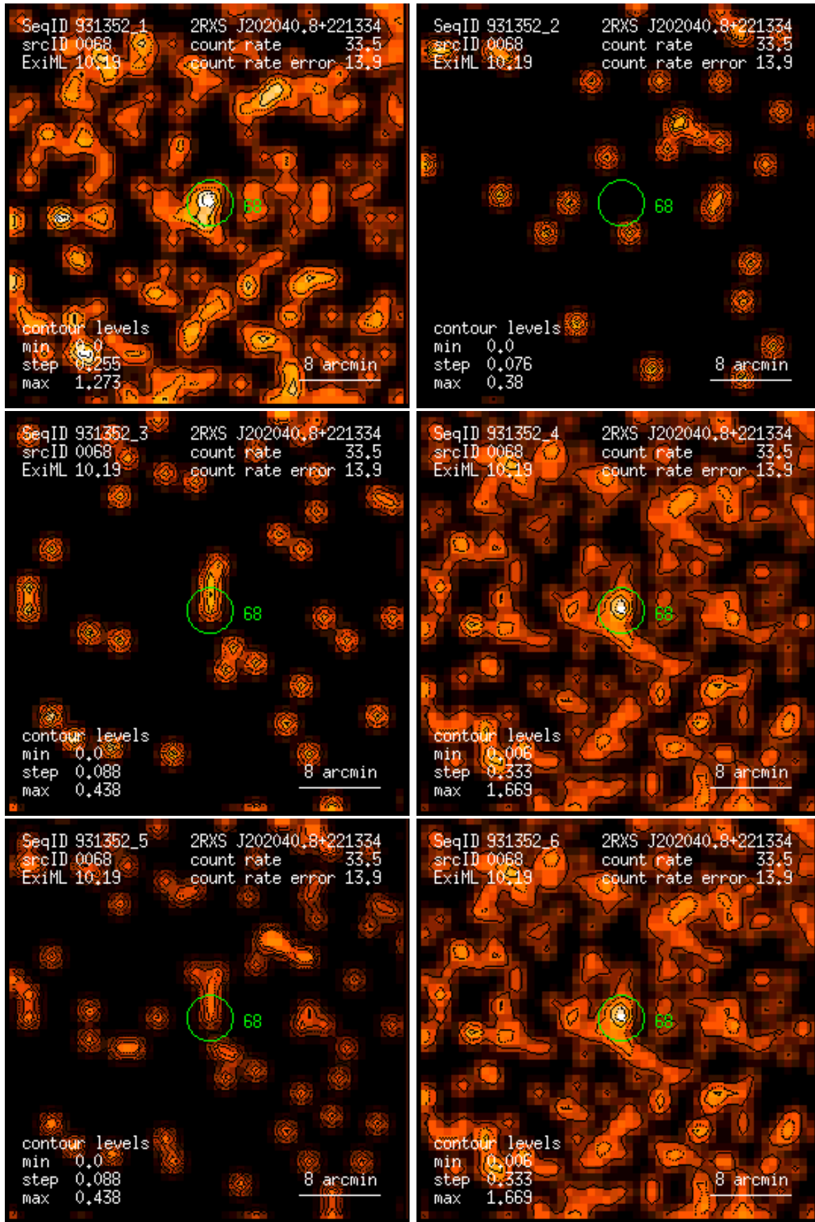
Figure 68: RASS 931352: detection 0068: band rate images, Gaussian filter: (1) PSPC channels 11 – 41, (2) 52 – 90, (3) 91 – 201, (4) 11 – 235, (5) 52 – 201, (6) 11 – 201. Broad band rates in counts/ks. Band rate contour levels in counts/ks/arcmin 2 .
