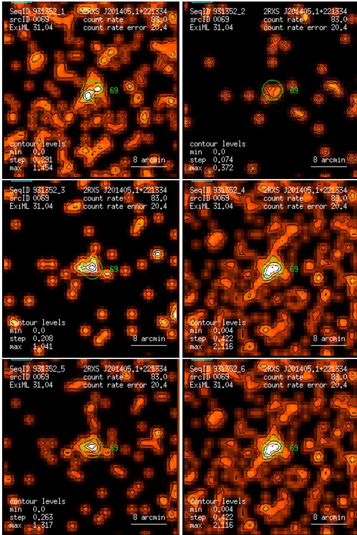
Figure 69: RASS 931352: detection 0069: band rate images, Gaussian filter: (1) PSPC channels 11 – 41, (2) 52 – 90, (3) 91 – 201, (4) 11 – 235, (5) 52 – 201, (6) 11 – 201. Broad band rates in counts/ks. Band rate contour levels in counts/ks/arcmin 2 .
