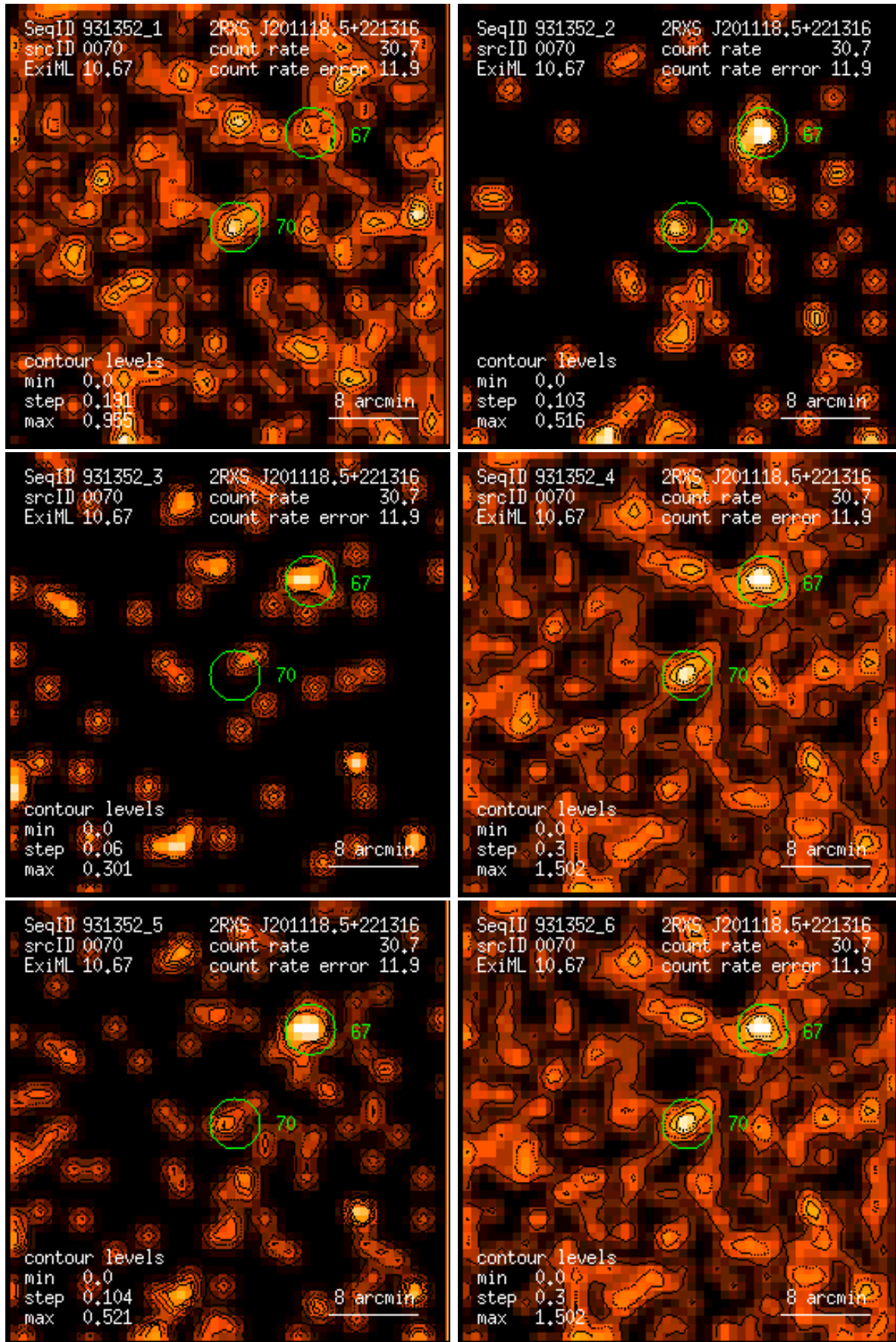
Figure 70: RASS 931352: detection 0070: band rate images, Gaussian filter: (1) PSPC channels 11 – 41, (2) 52 – 90, (3) 91 – 201, (4) 11 – 235, (5) 52 – 201, (6) 11 – 201. Broad band rates in counts/ks. Band rate contour levels in counts/ks/arcmin 2 .
