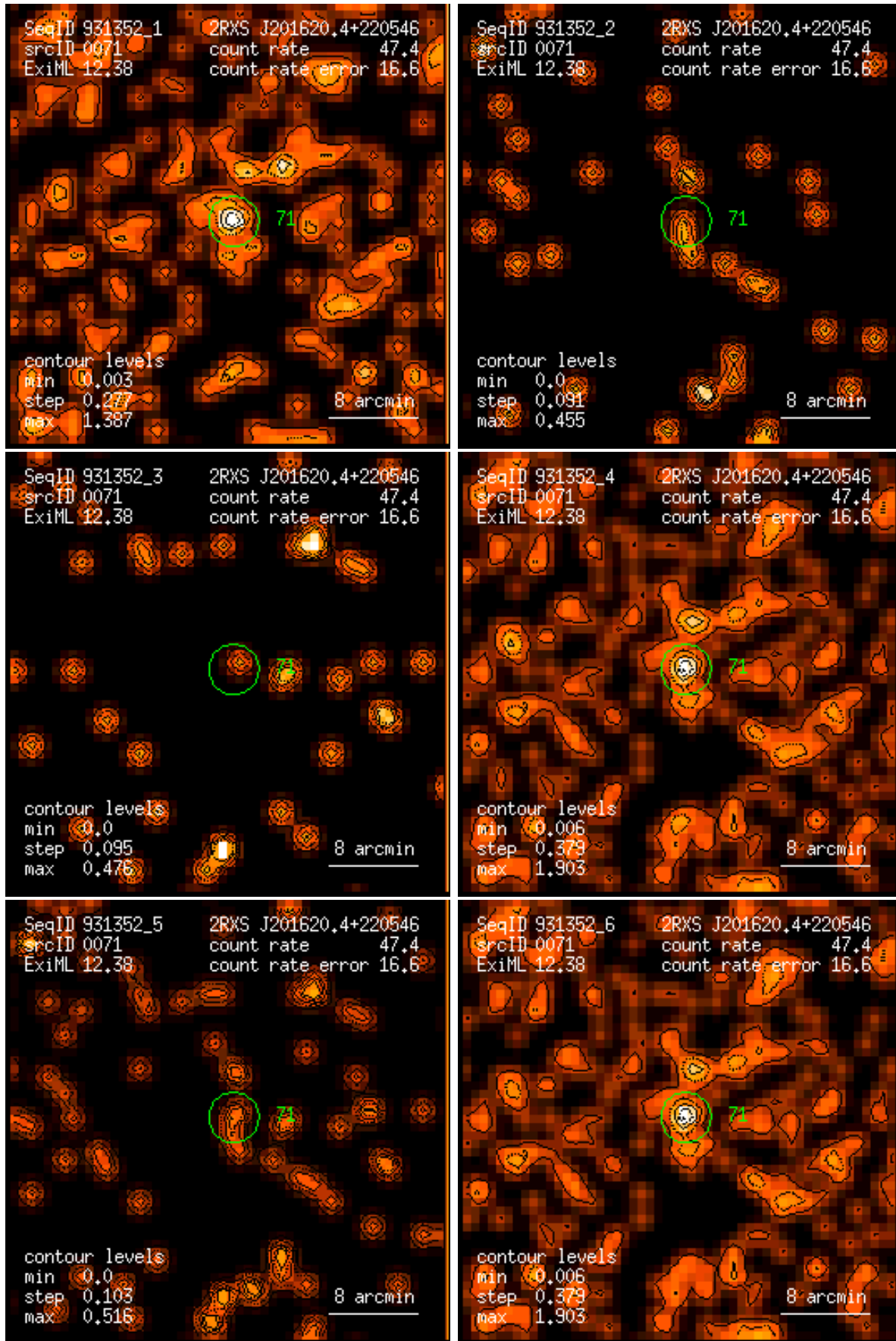
Figure 71: RASS 931352: detection 0071: band rate images, Gaussian filter: (1) PSPC channels 11 – 41, (2) 52 – 90, (3) 91 – 201, (4) 11 – 235, (5) 52 – 201, (6) 11 – 201. Broad band rates in counts/ks. Band rate contour levels in counts/ks/arcmin 2 .
