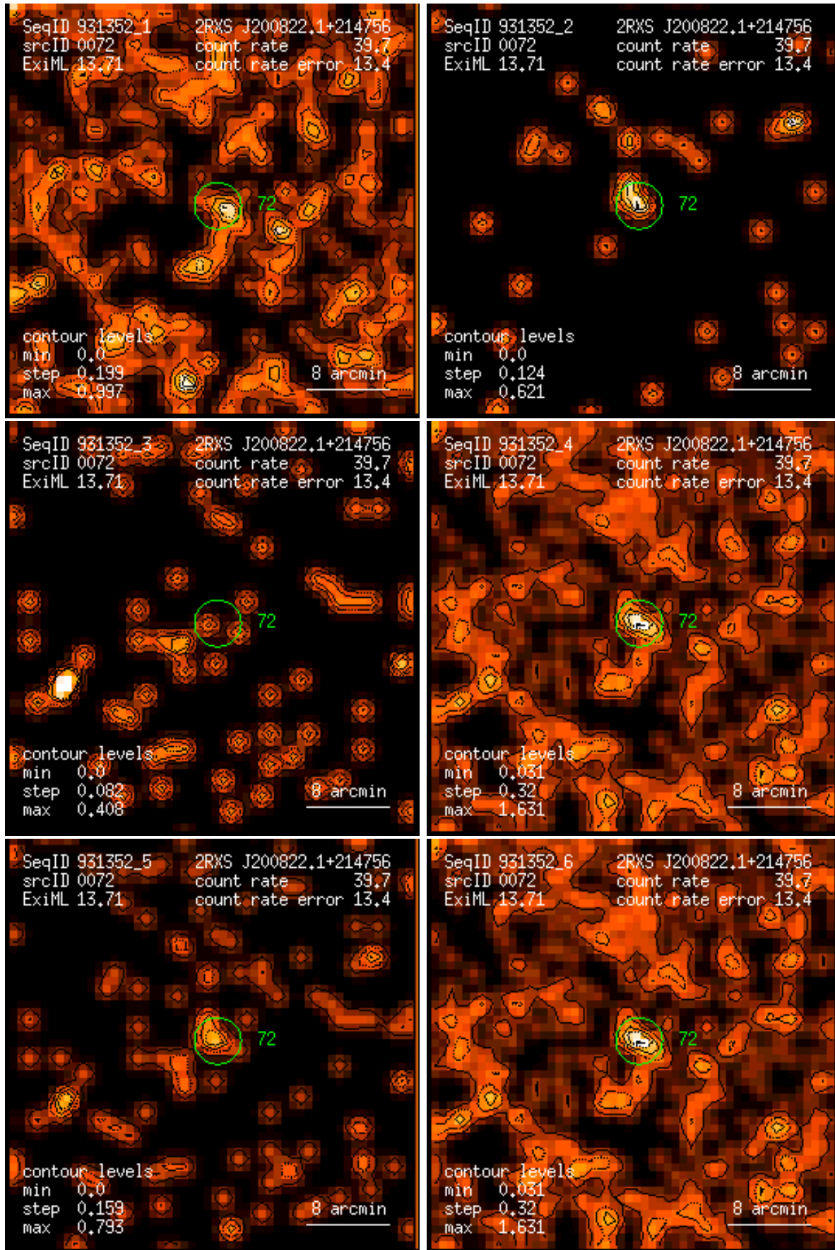
Figure 72: RASS 931352: detection 0072: band rate images, Gaussian filter: (1) PSPC channels 11 – 41, (2) 52 – 90, (3) 91 – 201, (4) 11 – 235, (5) 52 – 201, (6) 11 – 201. Broad band rates in counts/ks. Band rate contour levels in counts/ks/arcmin 2 .
