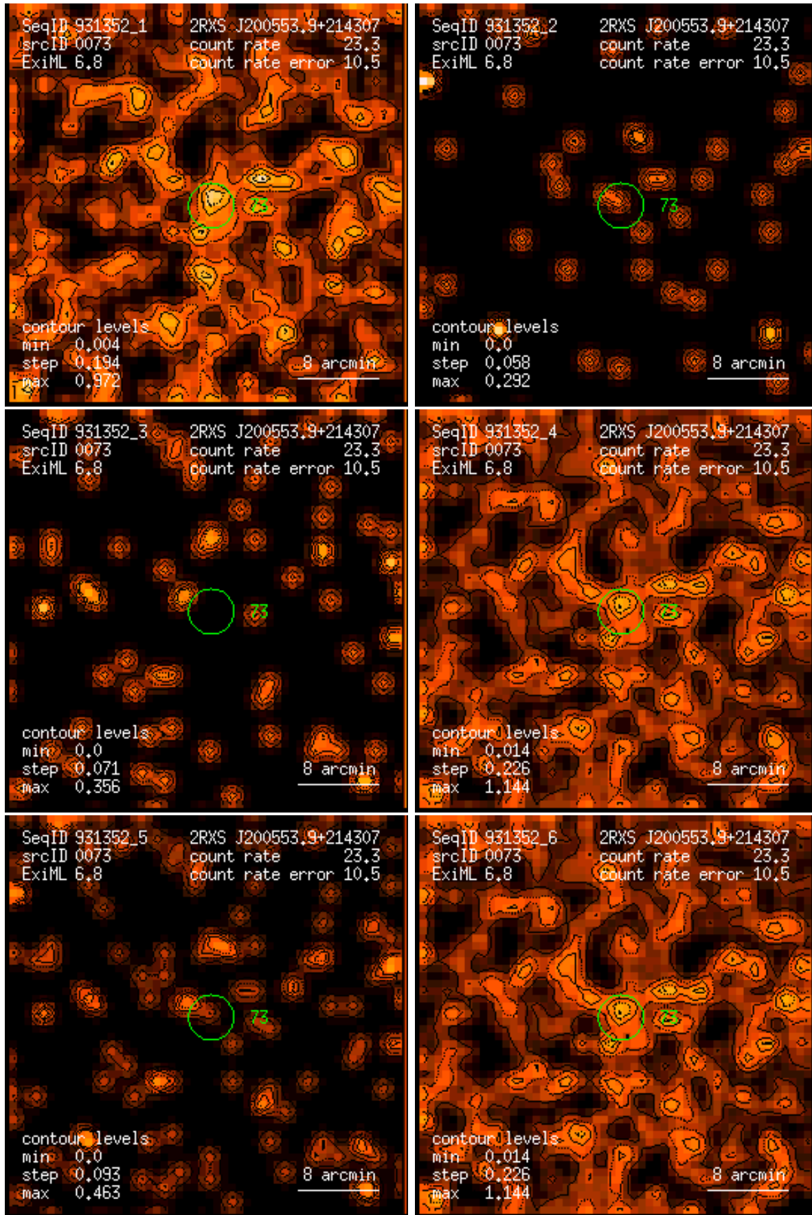
Figure 73: RASS 931352: detection 0073: band rate images, Gaussian filter: (1) PSPC channels 11 – 41, (2) 52 – 90, (3) 91 – 201, (4) 11 – 235, (5) 52 – 201, (6) 11 – 201. Broad band rates in counts/ks. Band rate contour levels in counts/ks/arcmin 2 .
