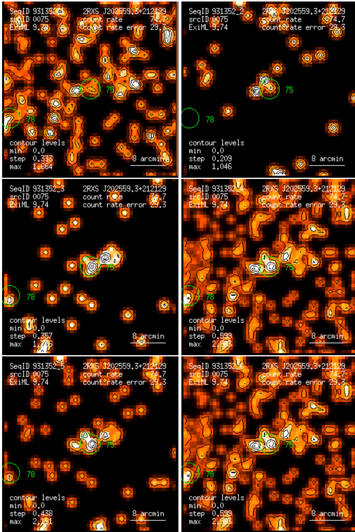
Figure 75: RASS 931352: detection 0075: band rate images, Gaussian filter: (1) PSPC channels 11 – 41, (2) 52 – 90, (3) 91 – 201, (4) 11 – 235, (5) 52 – 201, (6) 11 – 201. Broad band rates in counts/ks. Band rate contour levels in counts/ks/arcmin 2 .
