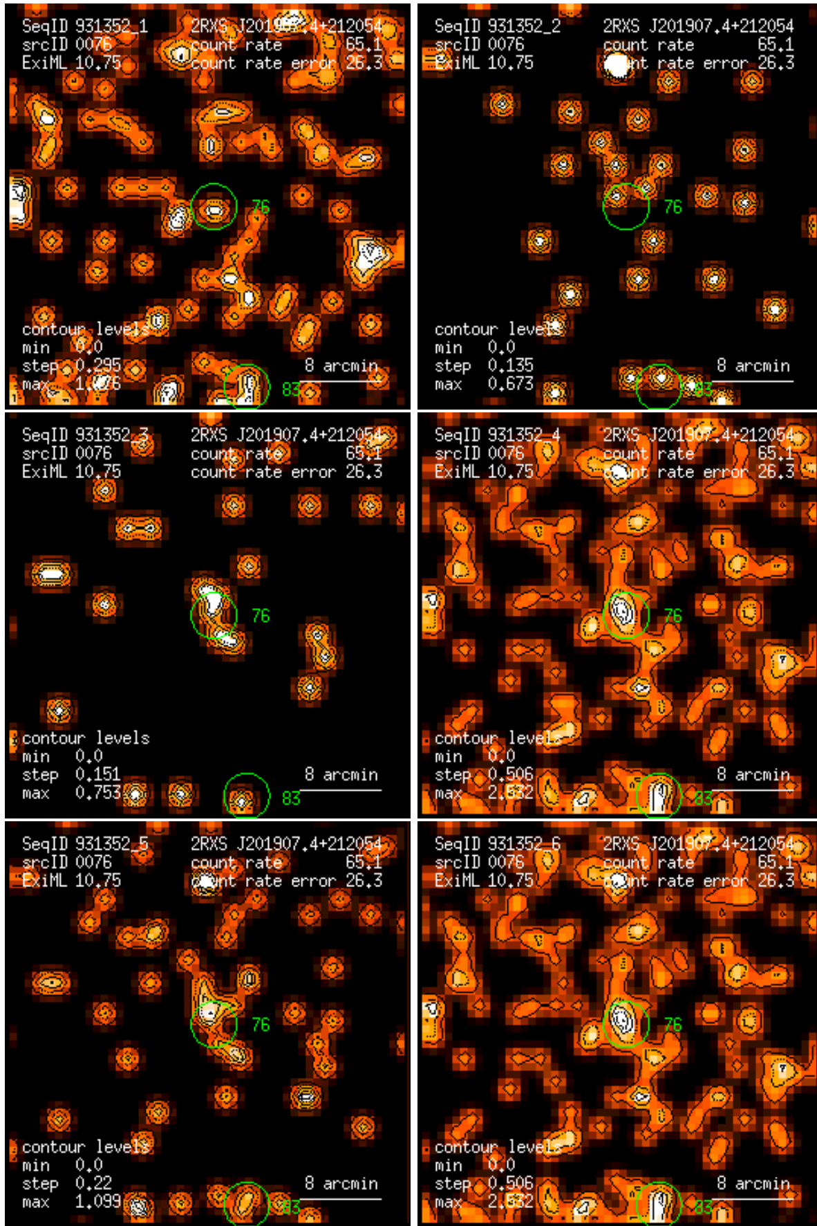
Figure 76: RASS 931352: detection 0076: band rate images, Gaussian filter: (1) PSPC channels 11 – 41, (2) 52 – 90, (3) 91 – 201, (4) 11 – 235, (5) 52 – 201, (6) 11 – 201. Broad band rates in counts/ks. Band rate contour levels in counts/ks/arcmin 2 .
