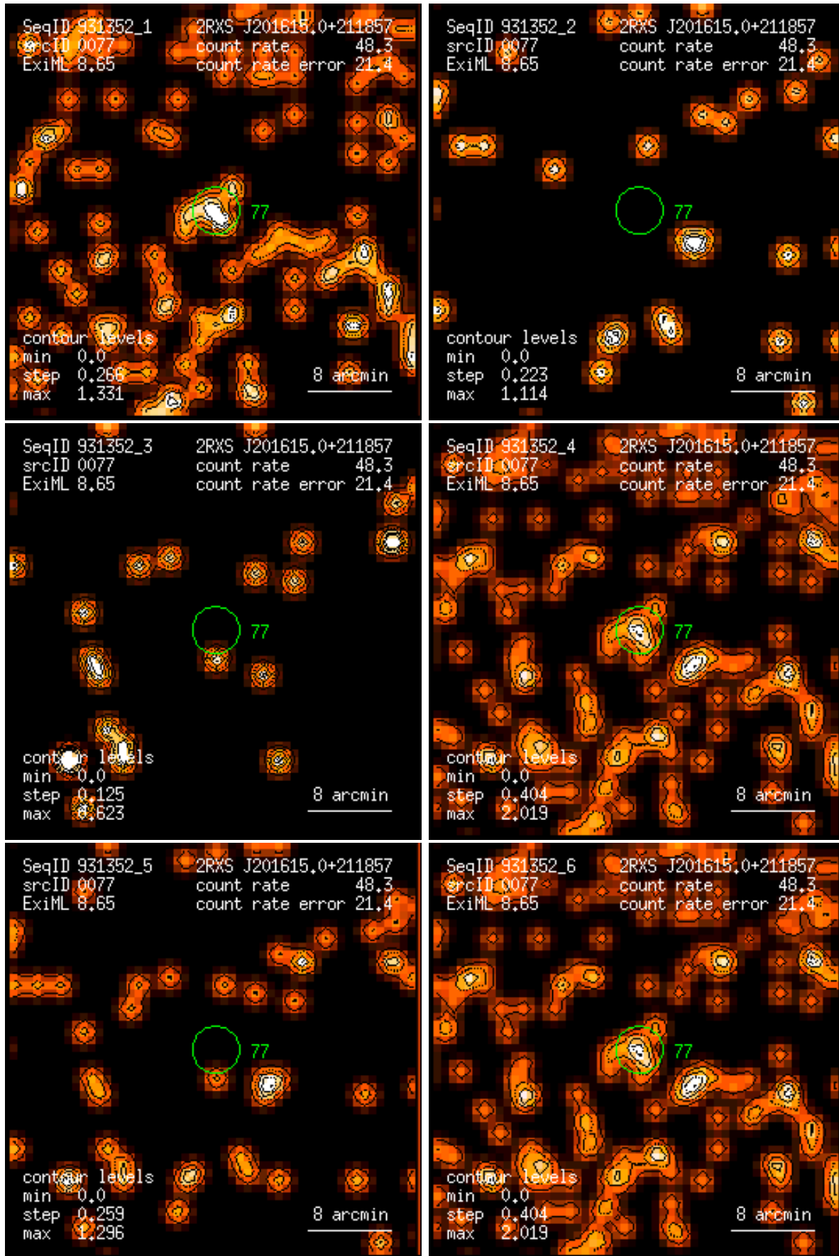
Figure 77: RASS 931352: detection 0077: band rate images, Gaussian filter: (1) PSPC channels 11 – 41, (2) 52 – 90, (3) 91 – 201, (4) 11 – 235, (5) 52 – 201, (6) 11 – 201. Broad band rates in counts/ks. Band rate contour levels in counts/ks/arcmin 2 .
