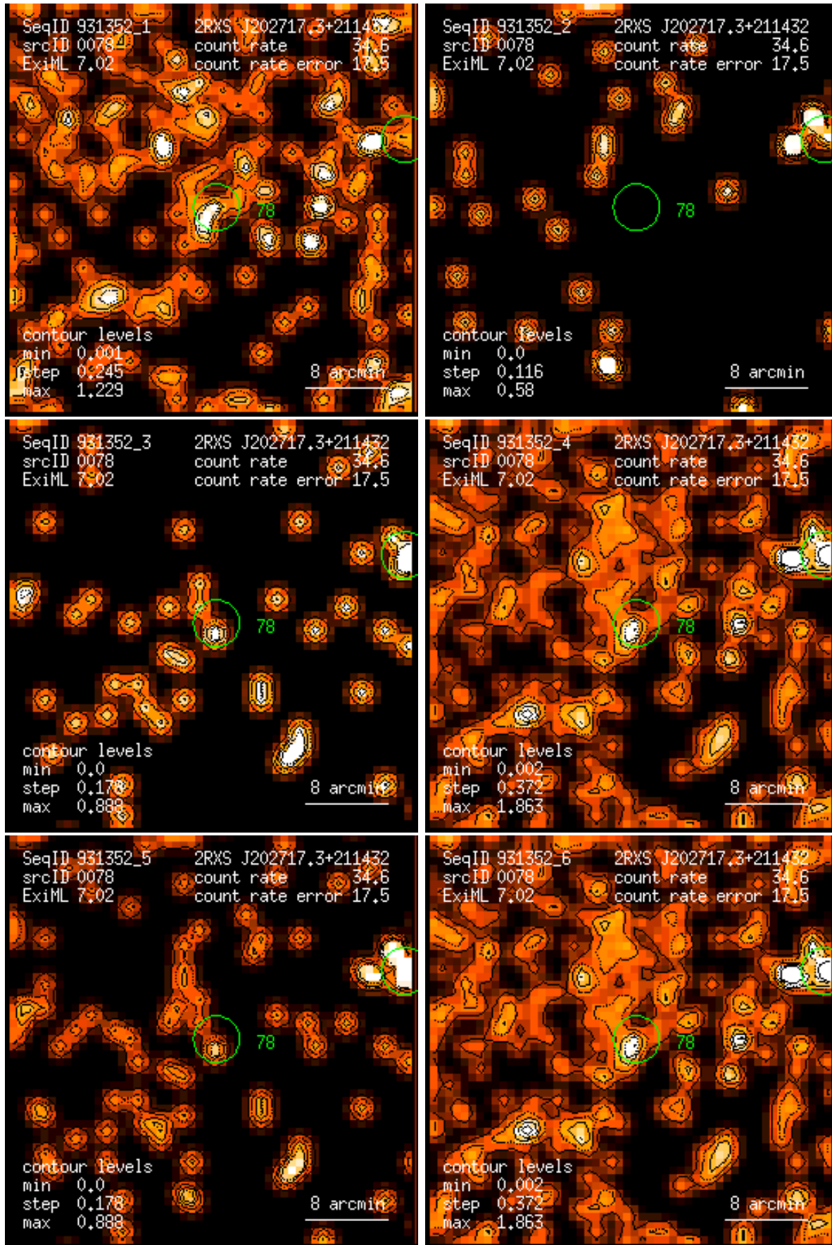
Figure 78: RASS 931352: detection 0078: band rate images, Gaussian filter: (1) PSPC channels 11 – 41, (2) 52 – 90, (3) 91 – 201, (4) 11 – 235, (5) 52 – 201, (6) 11 – 201. Broad band rates in counts/ks. Band rate contour levels in counts/ks/arcmin 2 .
