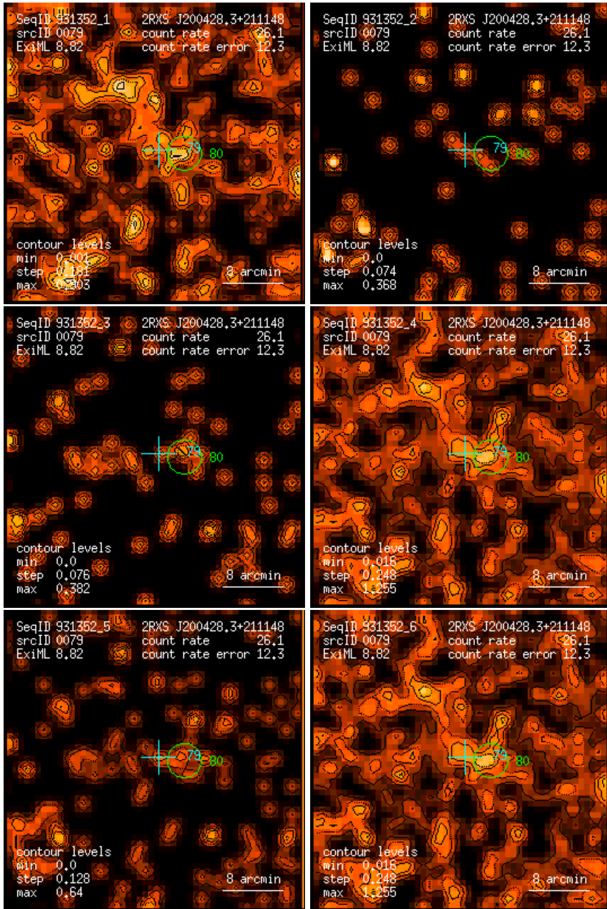
Figure 79: RASS 931352: detection 0079: band rate images, Gaussian filter: (1) PSPC channels 11 – 41, (2) 52 – 90, (3) 91 – 201, (4) 11 – 235, (5) 52 – 201, (6) 11 – 201. Broad band rates in counts/ks. Band rate contour levels in counts/ks/arcmin 2 .
