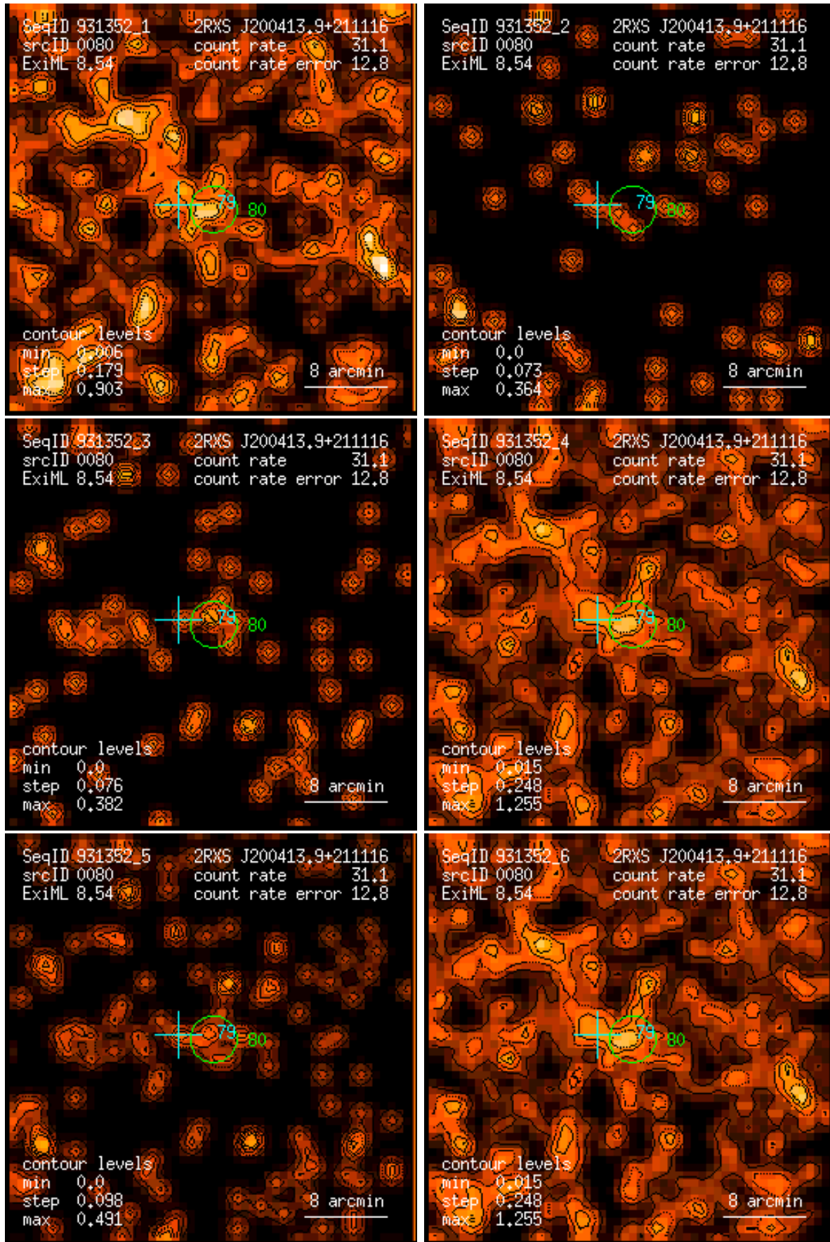
Figure 80: RASS 931352: detection 0080: band rate images, Gaussian filter: (1) PSPC channels 11 – 41, (2) 52 – 90, (3) 91 – 201, (4) 11 – 235, (5) 52 – 201, (6) 11 – 201. Broad band rates in counts/ks. Band rate contour levels in counts/ks/arcmin 2 .
