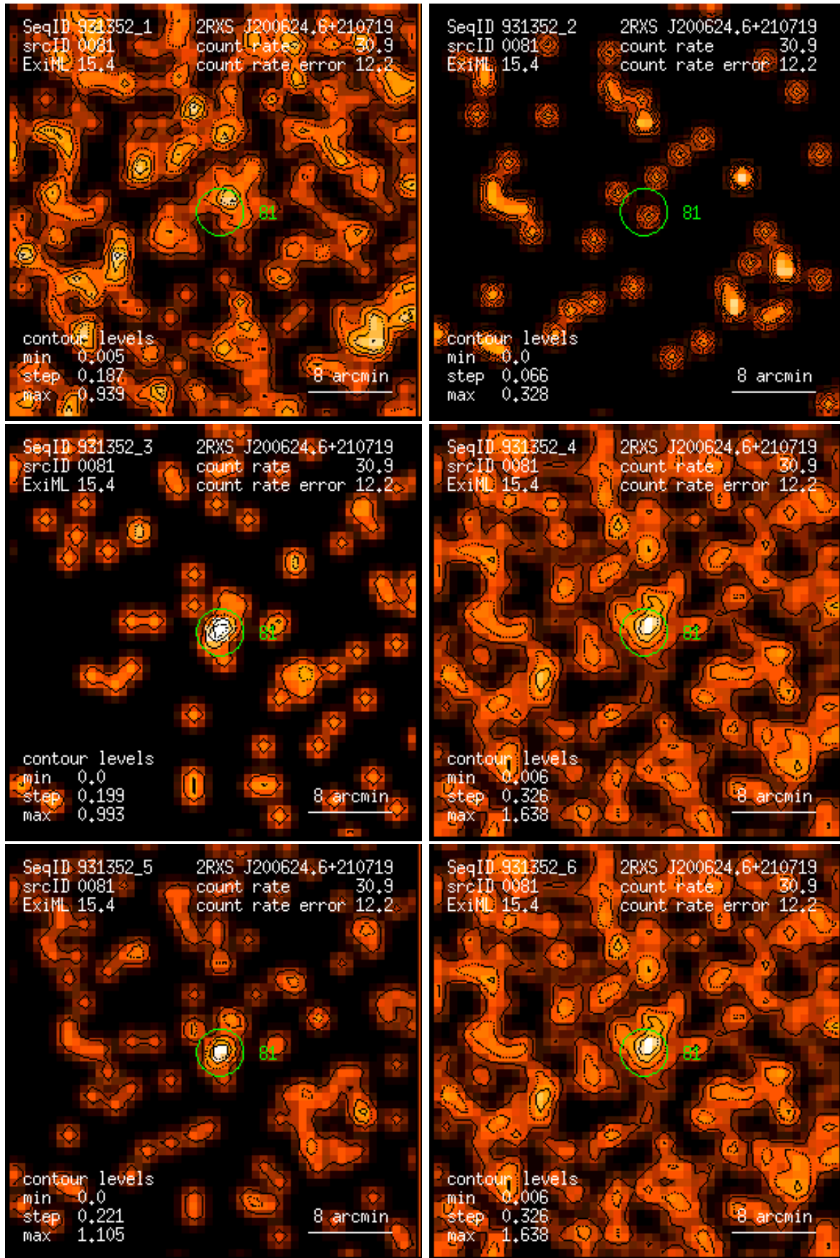
Figure 81: RASS 931352: detection 0081: band rate images, Gaussian filter: (1) PSPC channels 11 – 41, (2) 52 – 90, (3) 91 – 201, (4) 11 – 235, (5) 52 – 201, (6) 11 – 201. Broad band rates in counts/ks. Band rate contour levels in counts/ks/arcmin 2 .
