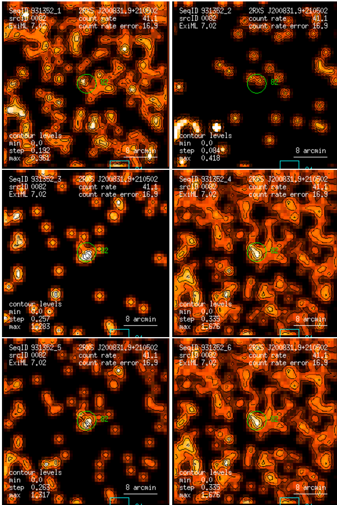
Figure 82: RASS 931352: detection 0082: band rate images, Gaussian filter: (1) PSPC channels 11 – 41, (2) 52 – 90, (3) 91 – 201, (4) 11 – 235, (5) 52 – 201, (6) 11 – 201. Broad band rates in counts/ks. Band rate contour levels in counts/ks/arcmin 2 .
