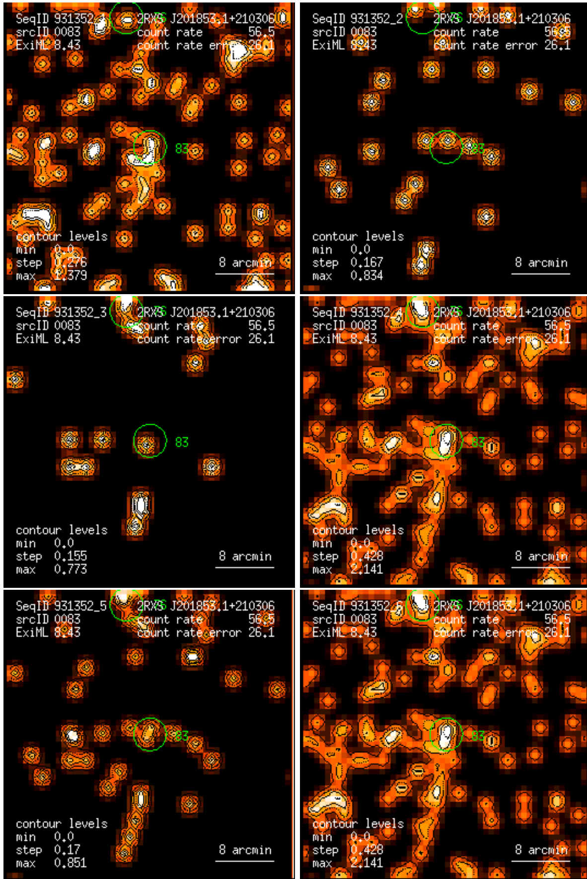
Figure 83: RASS 931352: detection 0083: band rate images, Gaussian filter: (1) PSPC channels 11 – 41, (2) 52 – 90, (3) 91 – 201, (4) 11 – 235, (5) 52 – 201, (6) 11 – 201. Broad band rates in counts/ks. Band rate contour levels in counts/ks/arcmin 2 .
