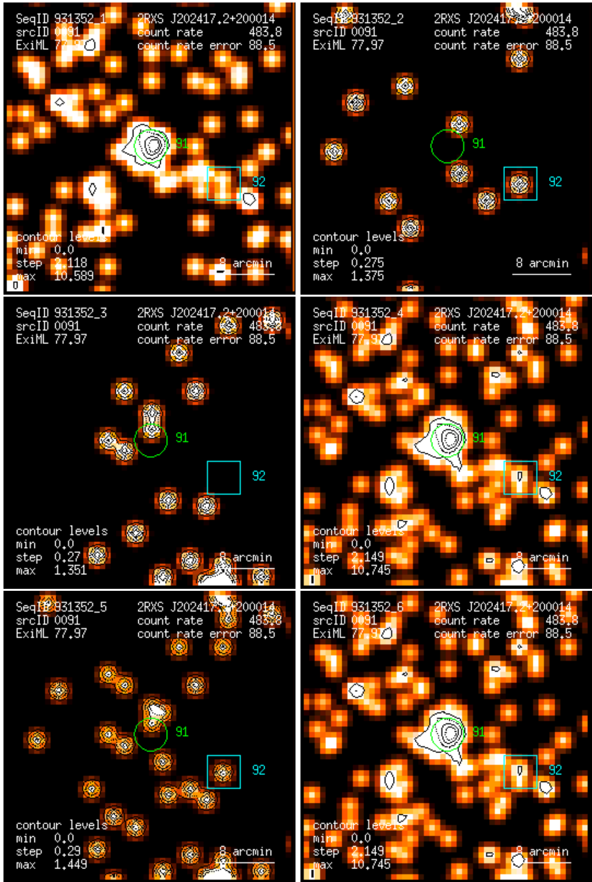
Figure 91: RASS 931352: detection 0091: band rate images, Gaussian filter: (1) PSPC channels 11 – 41, (2) 52 – 90, (3) 91 – 201, (4) 11 – 235, (5) 52 – 201, (6) 11 – 201. Broad band rates in counts/ks. Band rate contour levels in counts/ks/arcmin 2 .
