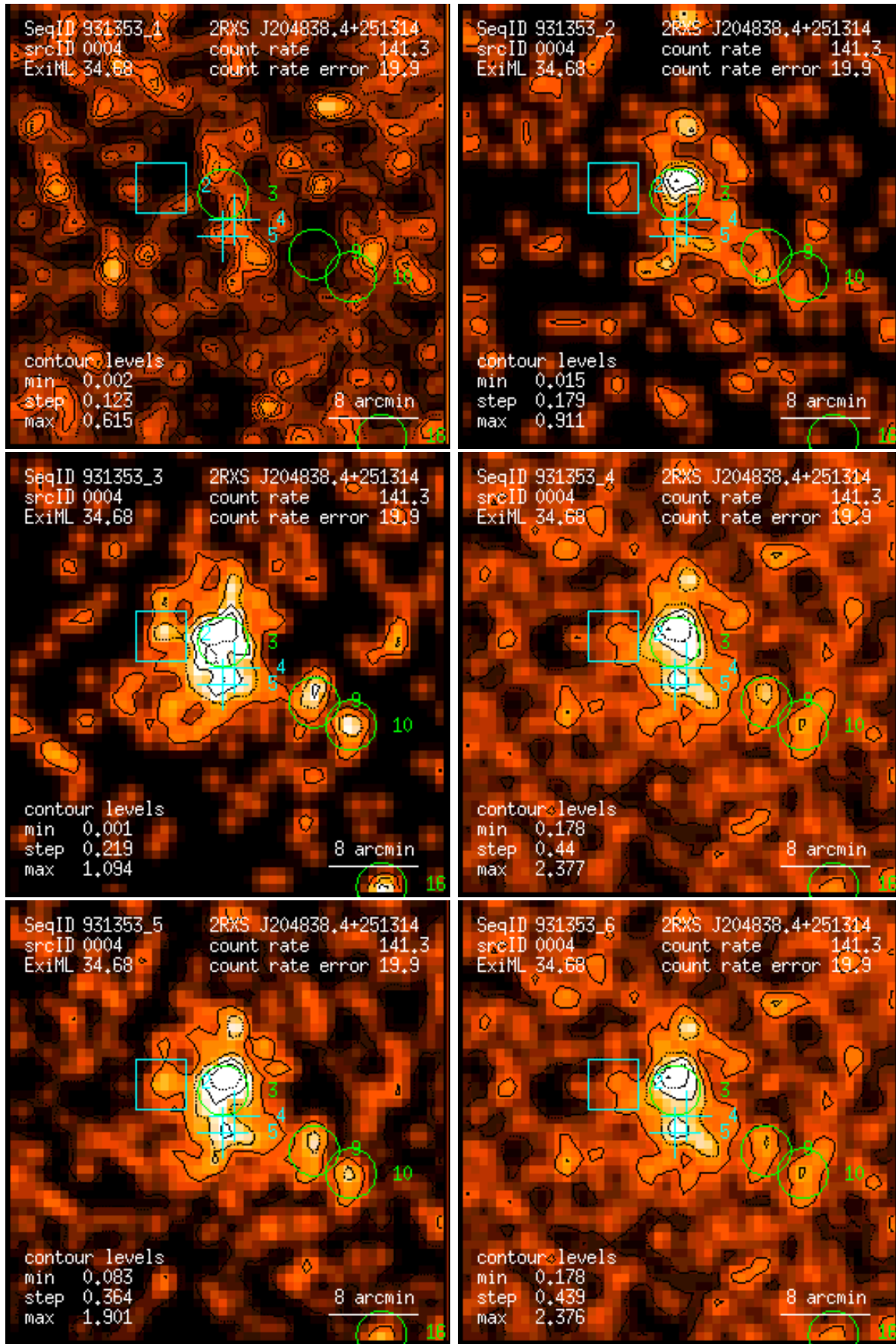
Figure 4: RASS 931353: detection 0004: band rate images, Gaussian filter: (1) PSPC channels 11 – 41, (2) 52 – 90, (3) 91 – 201, (4) 11 – 235, (5) 52 – 201, (6) 11 – 201. Broad band rates in counts/ks. Band rate contour levels in counts/ks/arcmin 2 .
