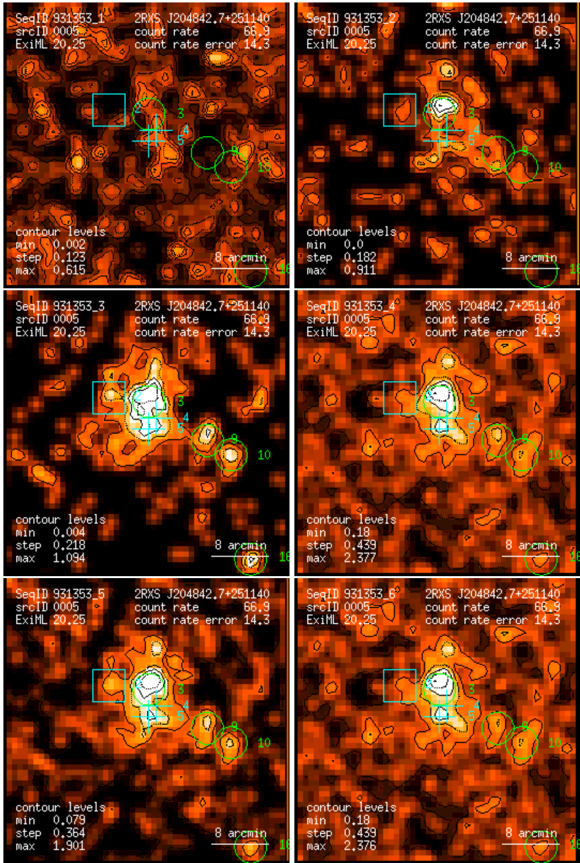
Figure 5: RASS 931353: detection 0005: band rate images, Gaussian filter: (1) PSPC channels 11 – 41, (2) 52 – 90, (3) 91 – 201, (4) 11 – 235, (5) 52 – 201, (6) 11 – 201. Broad band rates in counts/ks. Band rate contour levels in counts/ks/arcmin 2 .
