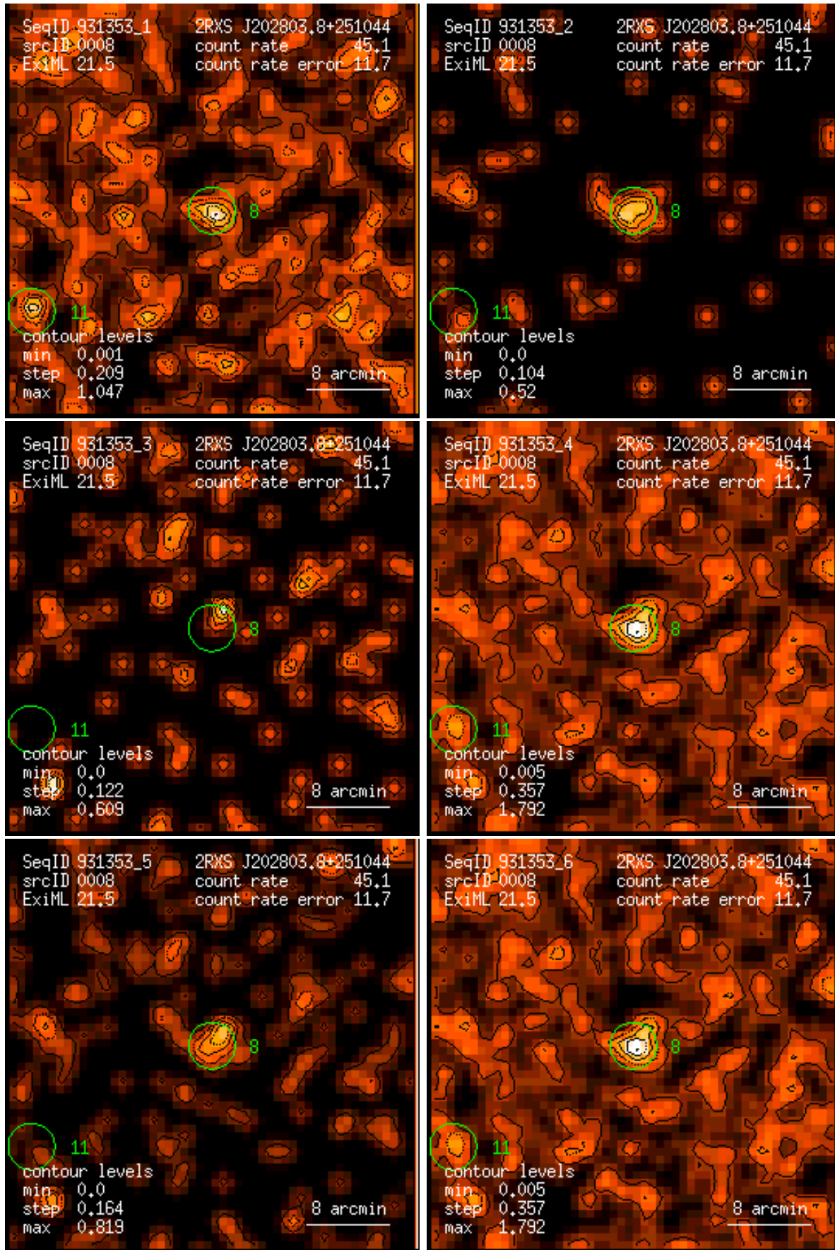
Figure 8: RASS 931353: detection 0008: band rate images, Gaussian filter: (1) PSPC channels 11 – 41, (2) 52 – 90, (3) 91 – 201, (4) 11 – 235, (5) 52 – 201, (6) 11 – 201. Broad band rates in counts/ks. Band rate contour levels in counts/ks/arcmin 2 .
