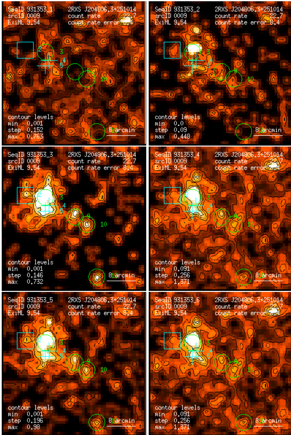
Figure 9: RASS 931353: detection 0009: band rate images, Gaussian filter: (1) PSPC channels 11 – 41, (2) 52 – 90, (3) 91 – 201, (4) 11 – 235, (5) 52 – 201, (6) 11 – 201. Broad band rates in counts/ks. Band rate contour levels in counts/ks/arcmin 2 .
