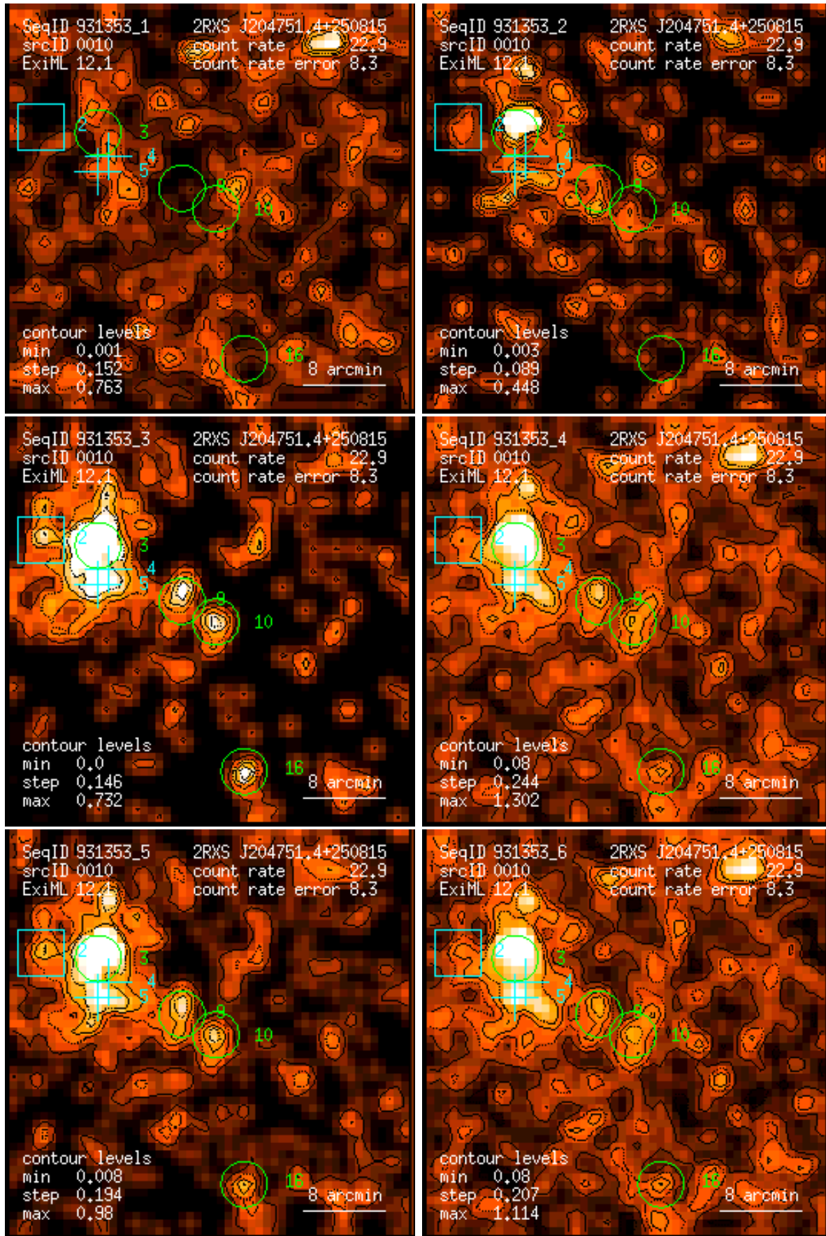
Figure 10: RASS 931353: detection 0010: band rate images, Gaussian filter: (1) PSPC channels 11 – 41, (2) 52 – 90, (3) 91 – 201, (4) 11 – 235, (5) 52 – 201, (6) 11 – 201. Broad band rates in counts/ks. Band rate contour levels in counts/ks/arcmin 2 .
