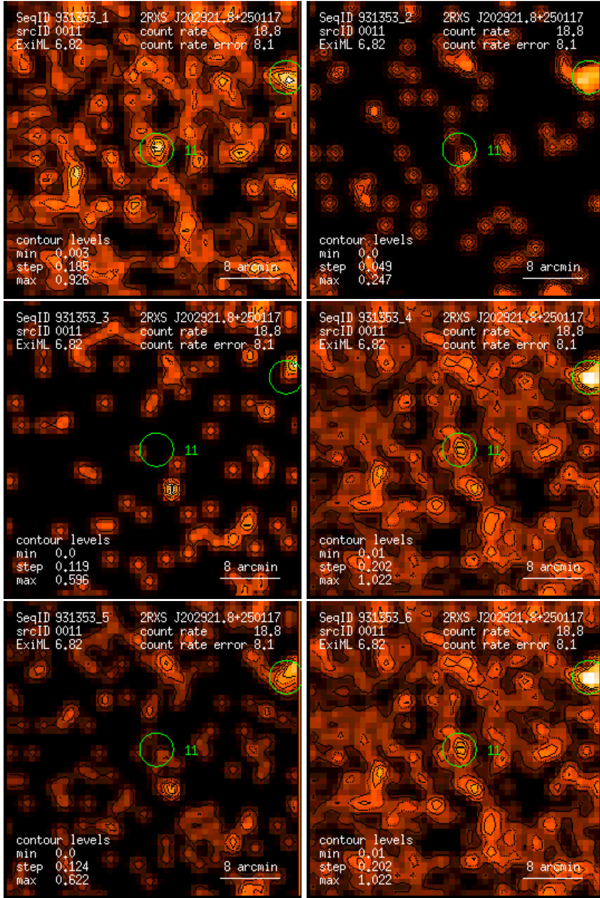
Figure 11: RASS 931353: detection 0011: band rate images, Gaussian filter: (1) PSPC channels 11 – 41, (2) 52 – 90, (3) 91 – 201, (4) 11 – 235, (5) 52 – 201, (6) 11 – 201. Broad band rates in counts/ks. Band rate contour levels in counts/ks/arcmin 2 .
