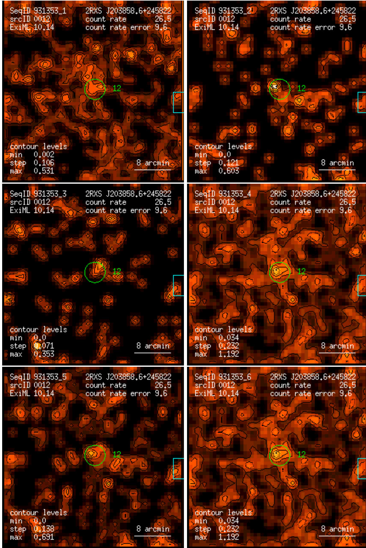
Figure 12: RASS 931353: detection 0012: band rate images, Gaussian filter: (1) PSPC channels 11 – 41, (2) 52 – 90, (3) 91 – 201, (4) 11 – 235, (5) 52 – 201, (6) 11 – 201. Broad band rates in counts/ks. Band rate contour levels in counts/ks/arcmin 2 .
