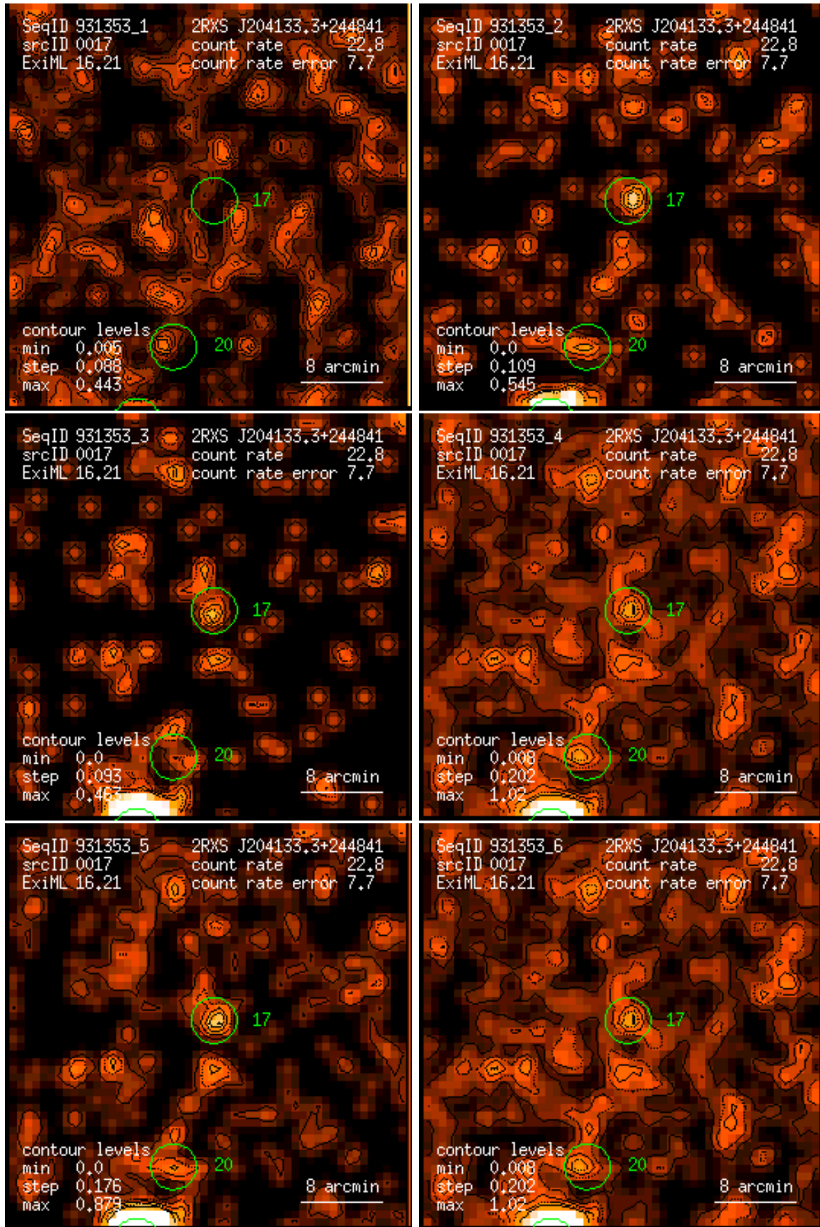
Figure 17: RASS 931353: detection 0017: band rate images, Gaussian filter: (1) PSPC channels 11 – 41, (2) 52 – 90, (3) 91 – 201, (4) 11 – 235, (5) 52 – 201, (6) 11 – 201. Broad band rates in counts/ks. Band rate contour levels in counts/ks/arcmin 2 .
